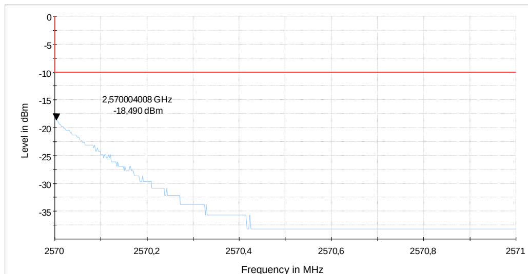
Diagram 63: 9.712b_SW2_LTE7_CH21400_BW10_RB1_HIGH_16QAM
