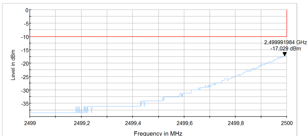
Diagram 54: 9.706a_SW1_LTE7_CH20825_BW15_RB75_LOW_QPSK
