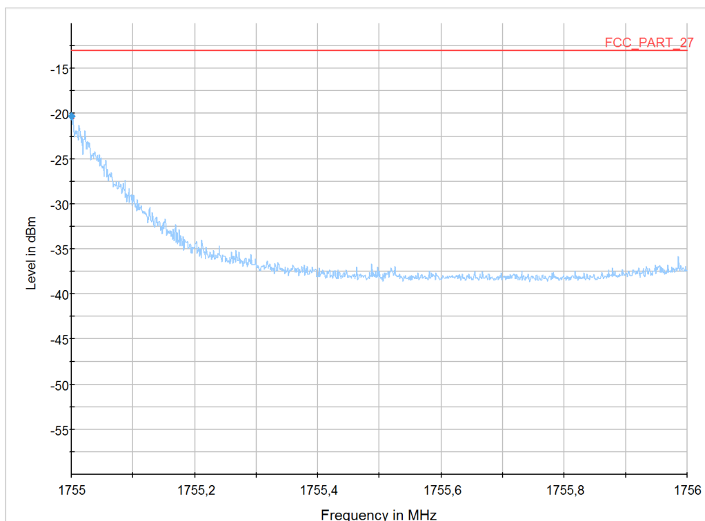
Diagram 27: 9.416a_LTE4_Ch20385_RB15high_BW3MHz_QPSK
