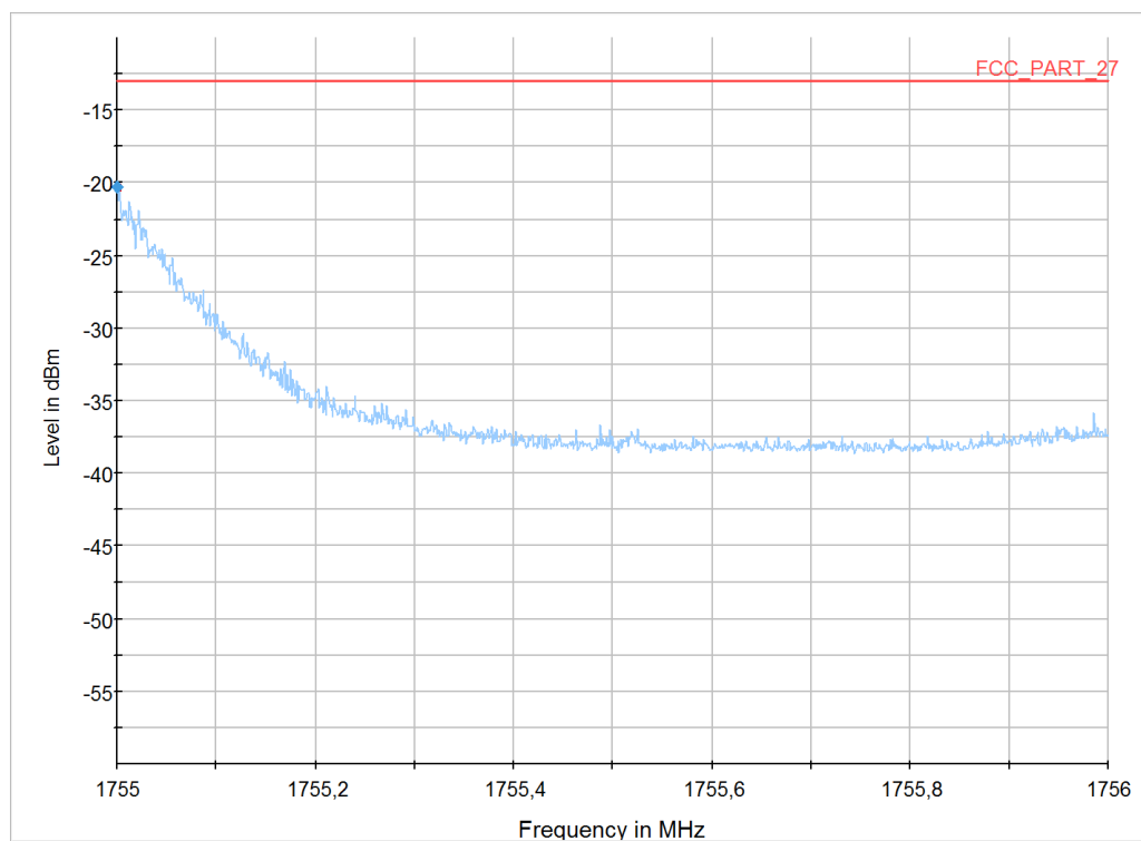
Diagram 26: 9.415b_LTE4_Ch20393_RB1high_BW3MHz_16QAM
