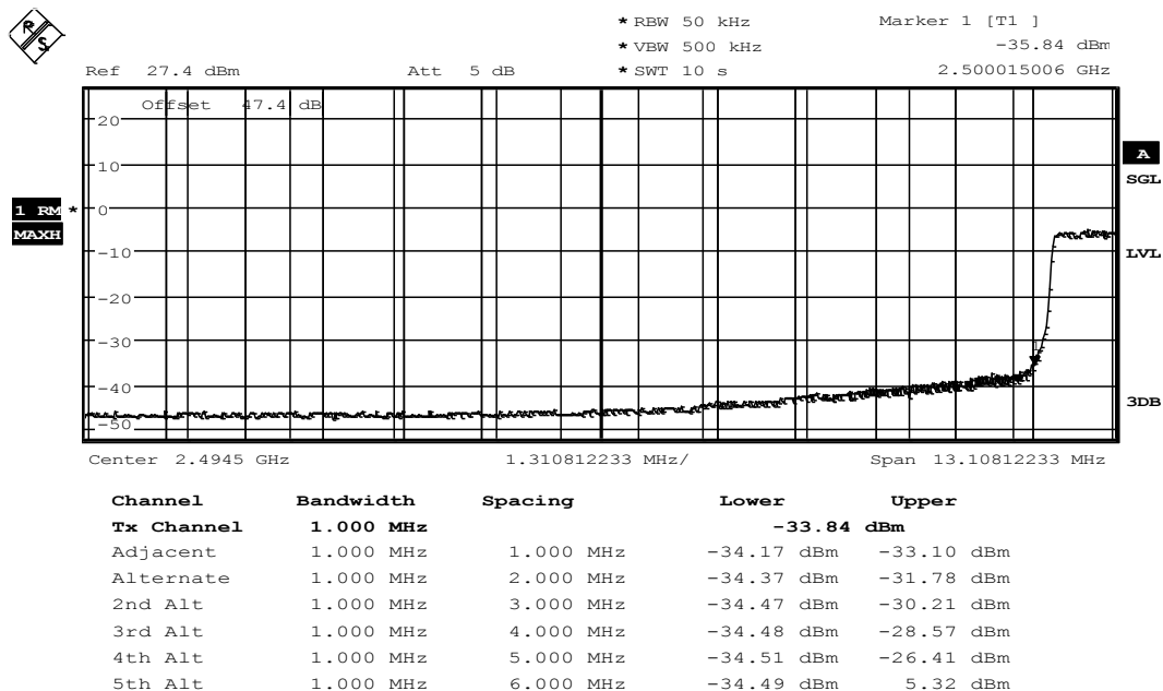
Diagram 47: 9.702b_SW1_LTE7_CH20775_BW5_RB25_LOW_16QAM_intBW
