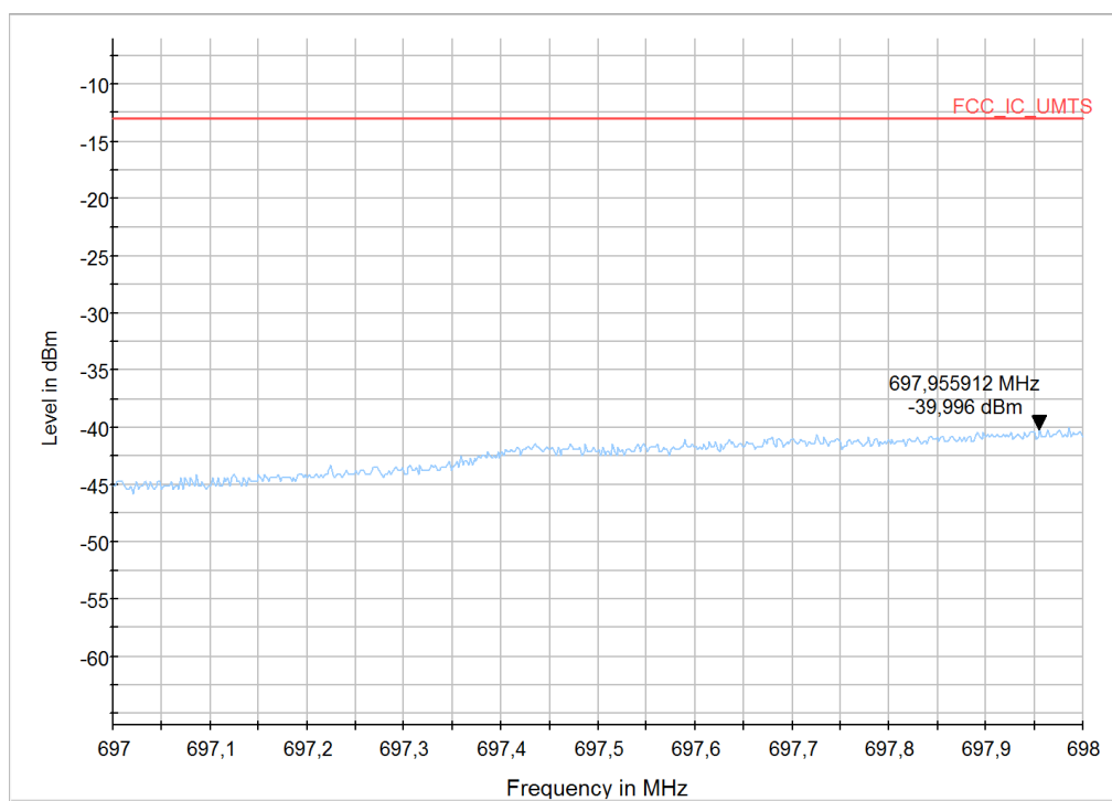
Diagram 71: 9.1204b_LTE12_CH23025_BW3_RB15low_16QAM
