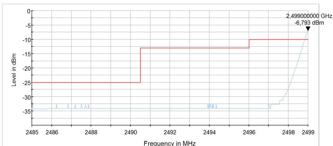
Diagram 51: 9.705b_SW1_LTE7_CH20825_BW15_RB1_LOW_16-QAM
