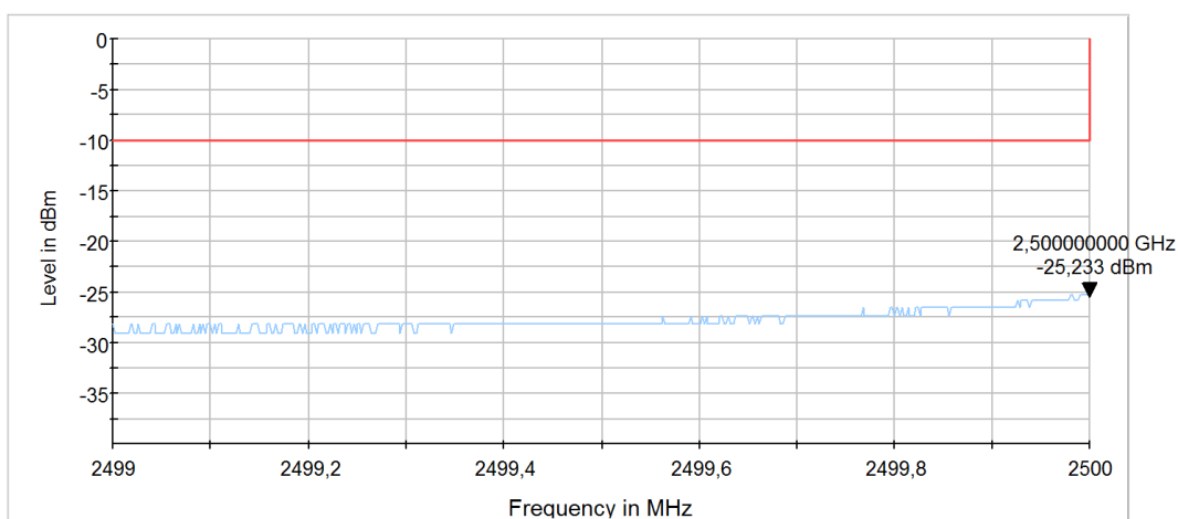
Diagram 55: 9.706a_SW2_LTE7_CH20825_BW15_RB75_LOW_QPSK
