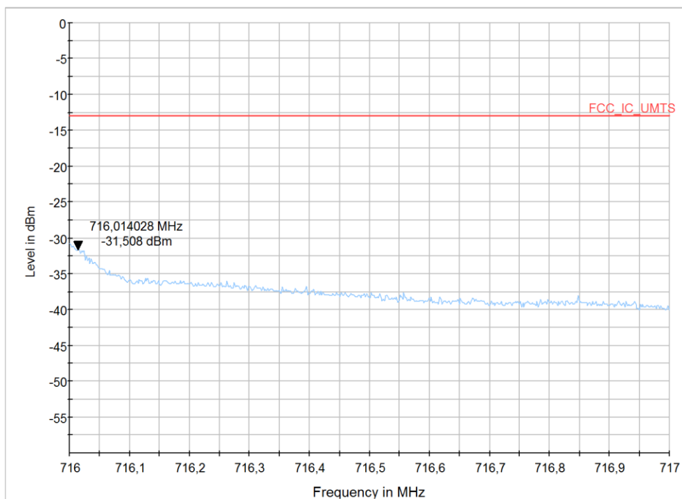
Diagram 74: 9.1212a_LTE12_CH23165_BW3_RB15high_QPSK
