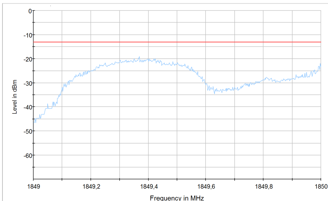
Diagram 1: 9.201a_LTE2_CH18607_BW1.4_RB1low_QPSK
