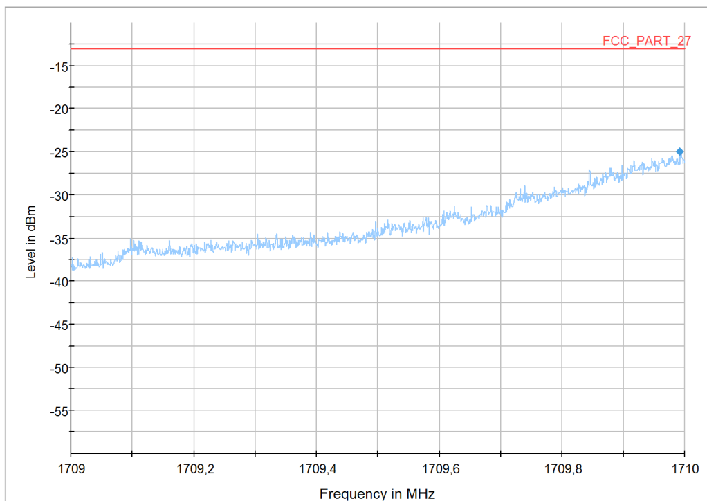
Diagram 16: 9.402b_LTE4_Ch19957_RB6low_BW1,4MHz_16QAM
