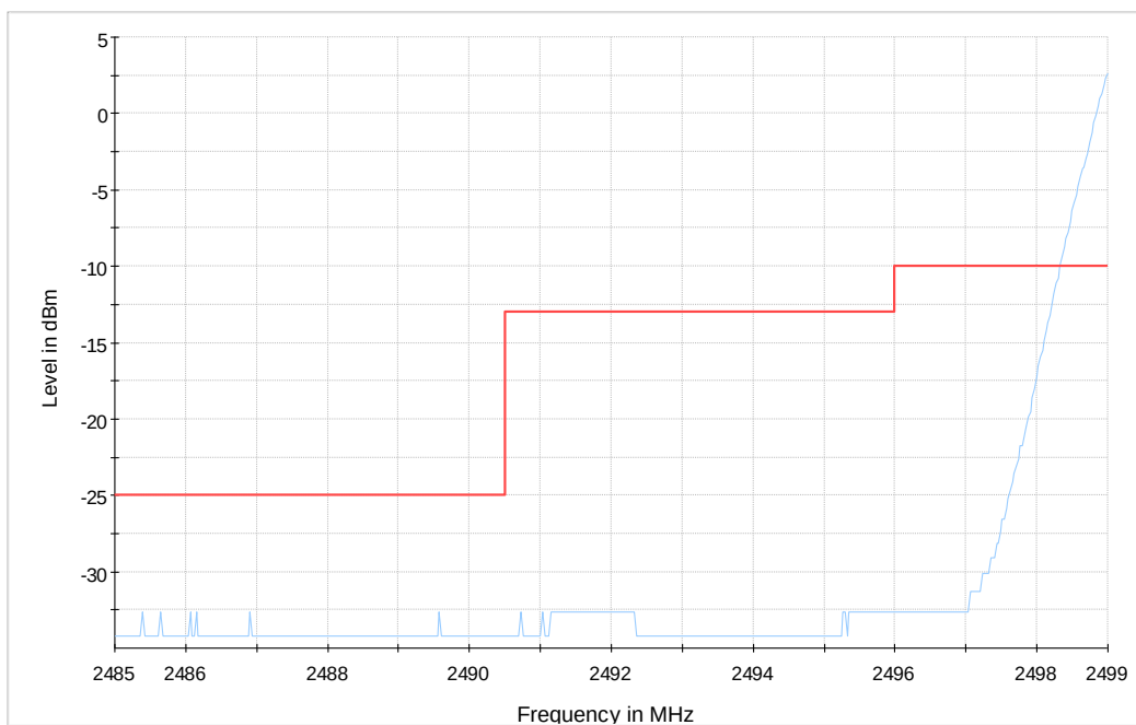
Diagram 40: 9.701b_SW1_LTE7_CH20775_BW5_RB1_LOW_16QAM
