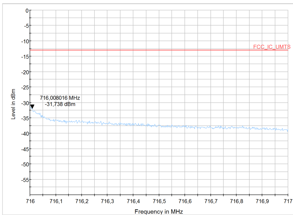
Diagram 75: 9.1212b_LTE12_CH23165_BW3_RB15high_16QAM
