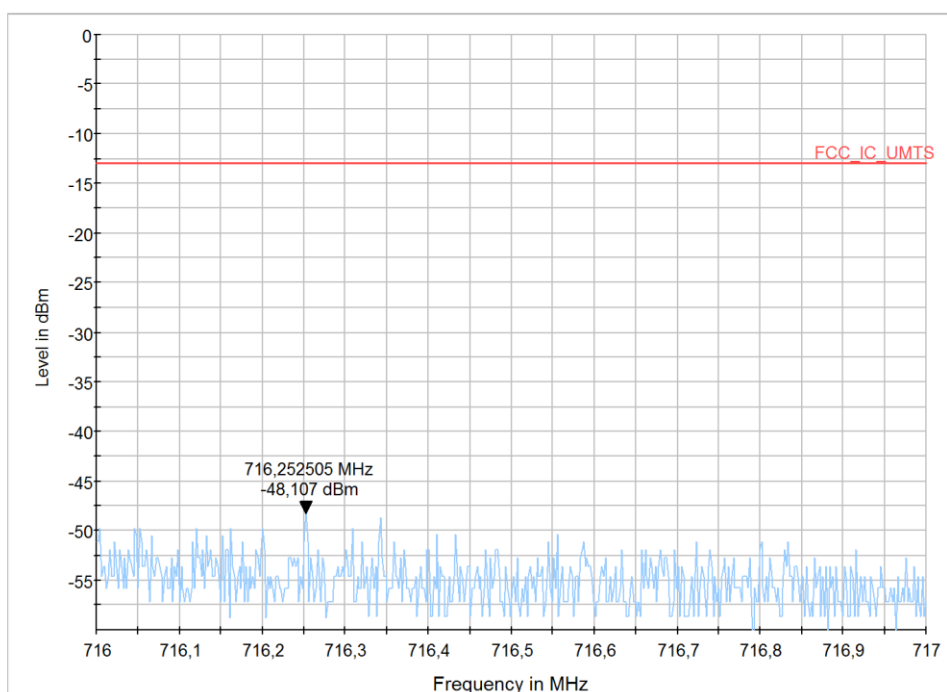
Diagram 73: 9.1211b_LTE12_CH23165_BW3_RB1high_16QAM
