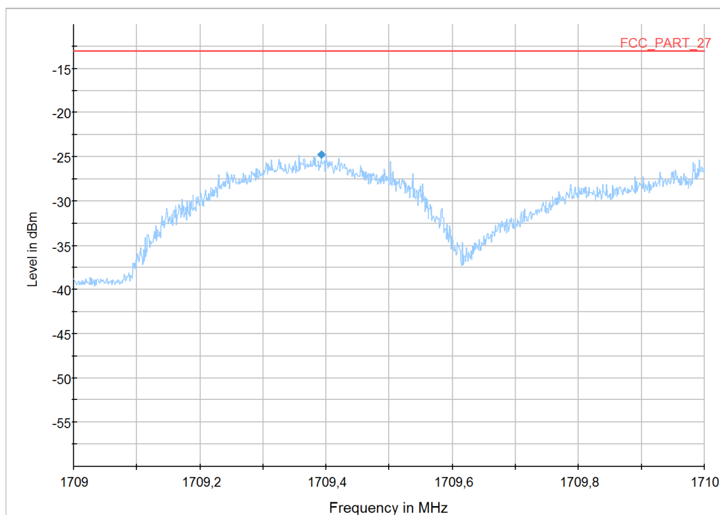
Diagram 14: 9.401b_LTE4_Ch19957_RB1low_BW1,4MHz_16QAM
