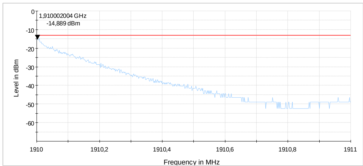
Diagram 10: 9.215b_LTE2_CH19185_BW3_RB1high_16QAM
