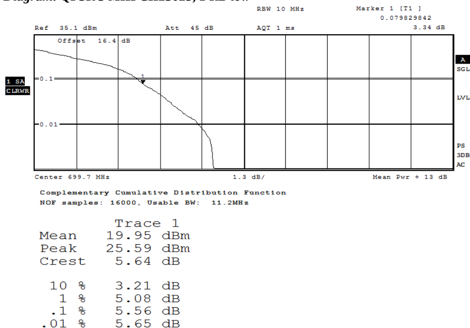
Diagram: 16QAM 3 MHz CH23025, 1 RB low
