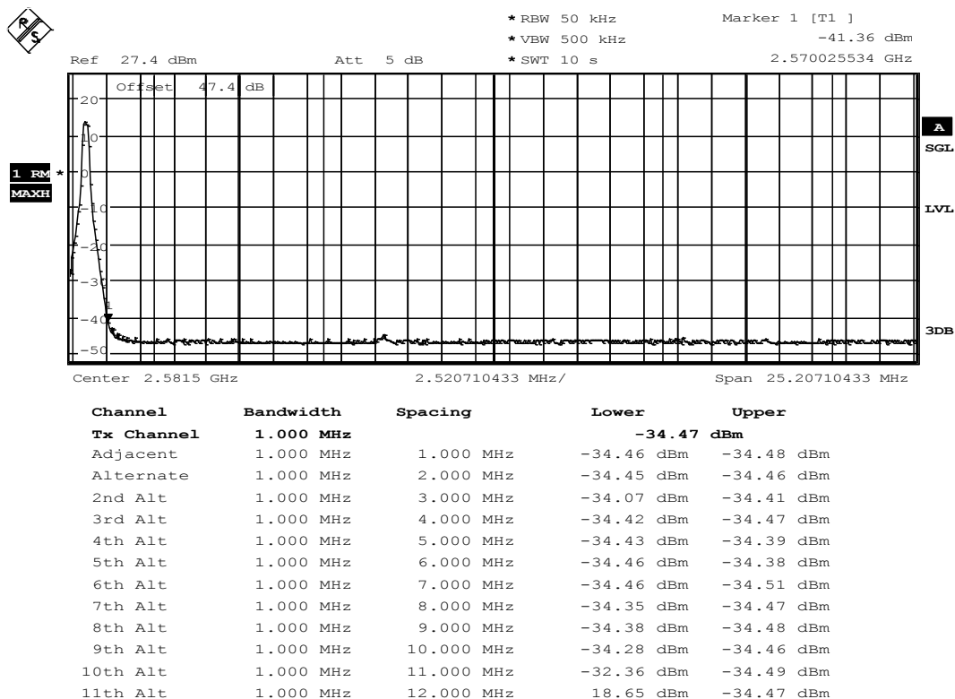
Diagram 62: 9.712b_SW1_LTE7_CH21400_BW10_RB1_HIGH_16_QAM_intBW
