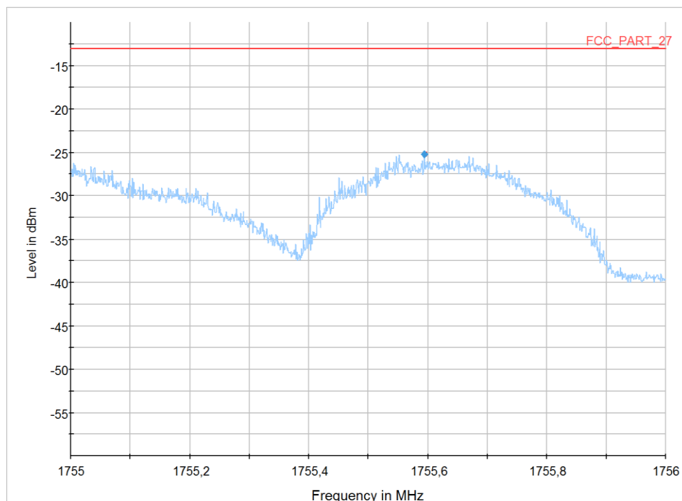
Diagram 22: 9.413b_LTE4_Ch20393_RB1high_BW1,4MHz_16QAM
