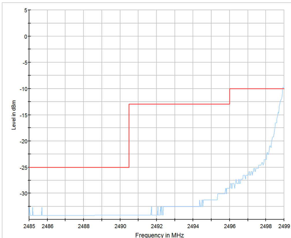
Diagram 46: 9.702b_SW1_LTE7_CH20775_BW5_RB25_LOW_16QAM
