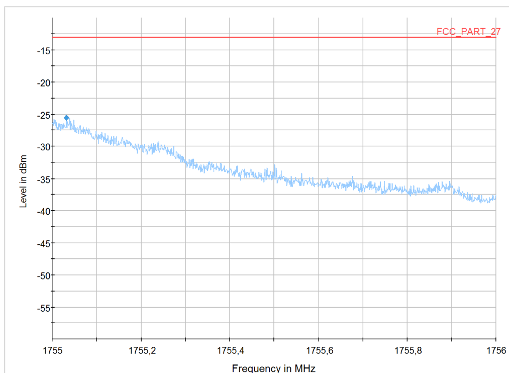
Diagram 24: 9.414b_LTE4_Ch20393_RB6high_BW1,4MHz_16QAM
