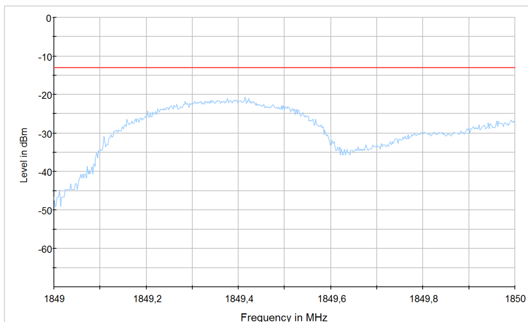
Diagram 2: 9.201b_LTE2_CH18607_BW1.4_RB1low_16-QAM
