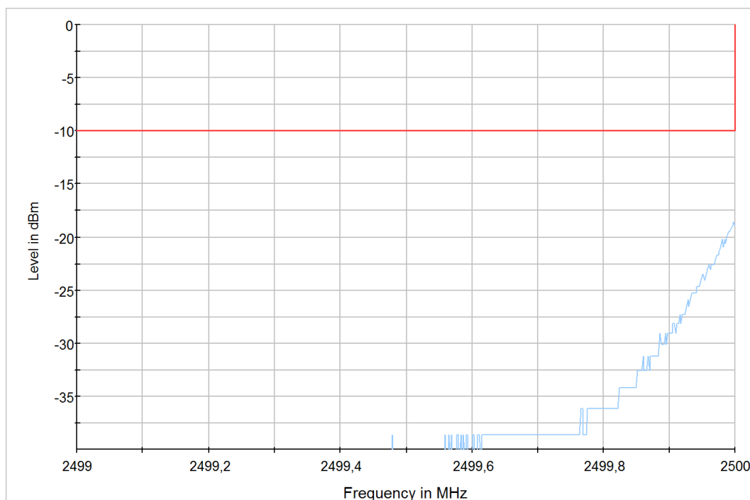
Diagram 42: 9.701b_SW2_LTE7_CH20775_BW5_RB1_LOW_16QAM
