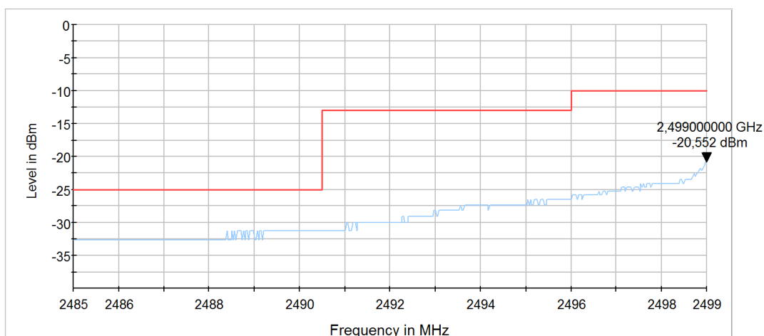
Diagram 57: 9.707b_SW2_LTE7_CH20825_BW15_RB75_LOW_16QAM
