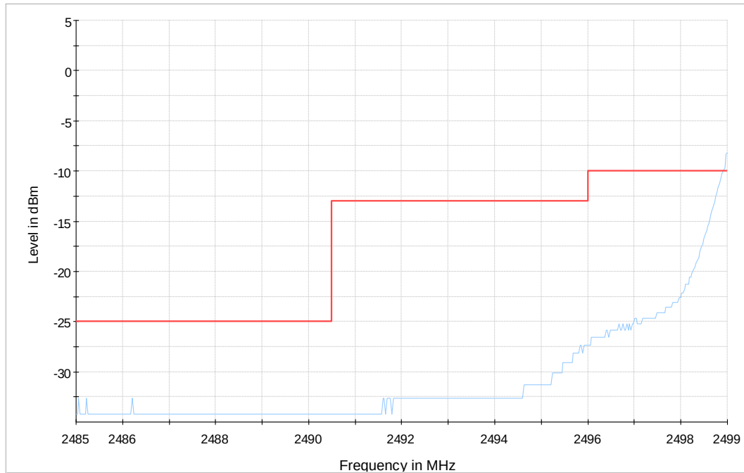
Diagram 43: 9.702a_SW1_LTE7_CH20775_BW5_RB25_LOW_QPSK
