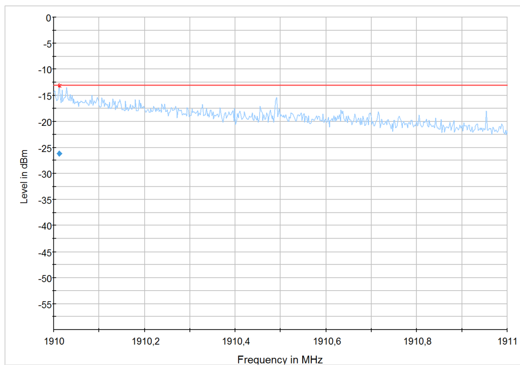
Diagram 12: 9.216b_LTE2_CH19185_BW3_RB15high_16-QAM
