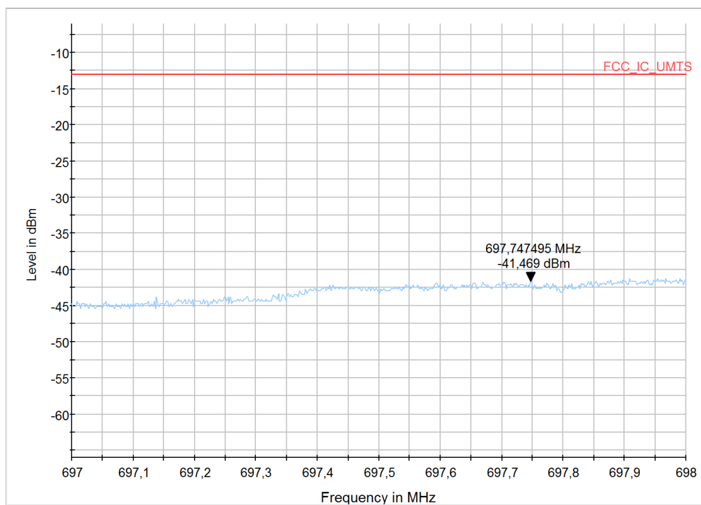
Diagram 70: 9.1204a_LTE12_CH23025_BW3_RB15low_QPSK
