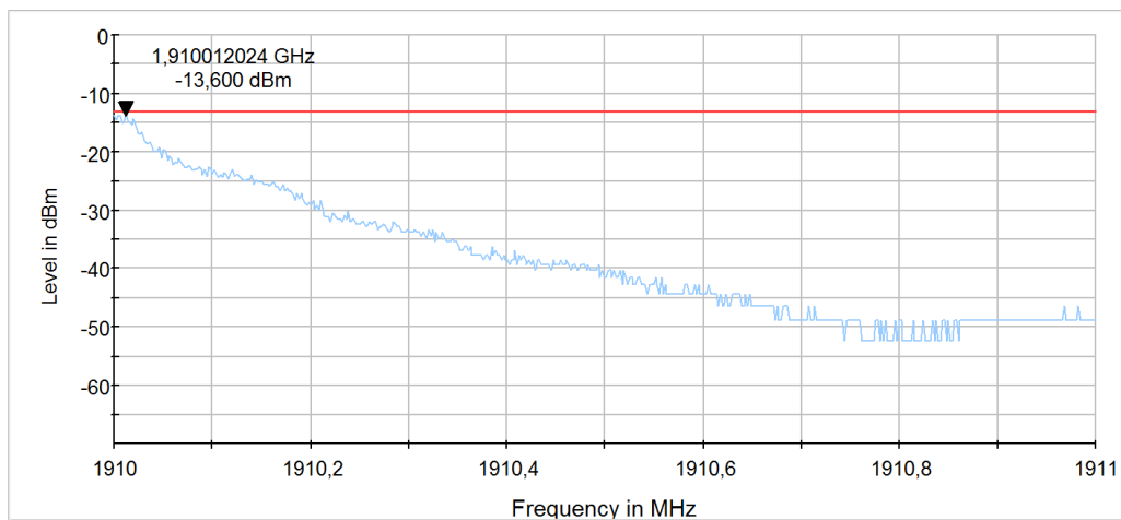
Diagram 9: 9.215a_LTE2_CH19185_BW3_RB1high_QPSK
