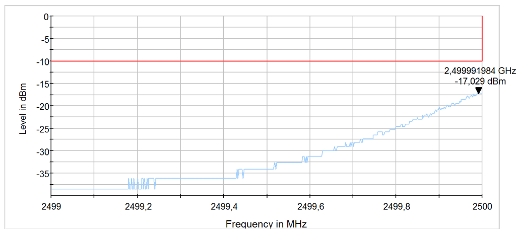
Diagram 53: 9.705b_SW2_LTE7_CH20825_BW15_RB1_LOW_16-QAM
