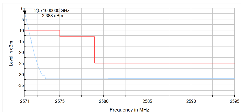
Diagram 61: 9.712b_SW1_LTE7_CH21400_BW10_RB1_HIGH_16QAM
