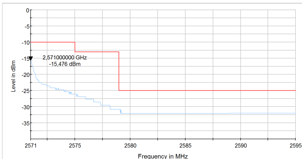
Diagram 64: 9.713a_SW1_LTE7_CH21400_BW10_RB1_HIGH_QPSK
