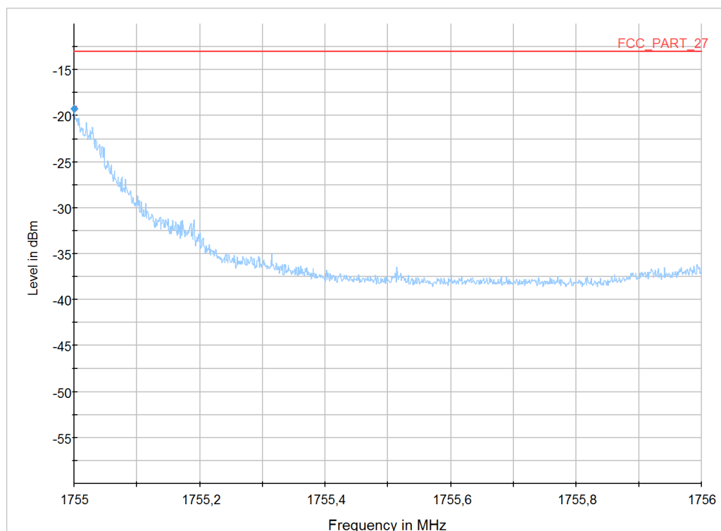
Diagram 25: 9.415a_LTE4_Ch20385_RB1high_BW3MHz_QPSK
