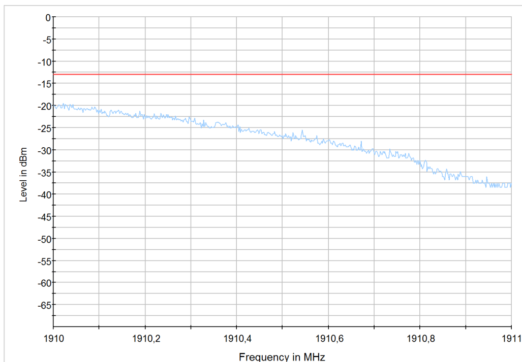
Diagram 6: 9.213b_LTE2_CH19193_BW1,4_RB6high_16QAM
