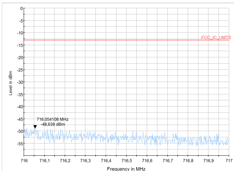
Diagram 72: 9.1210a_LTE12_CH23165_BW3_RB1high_QPSK
