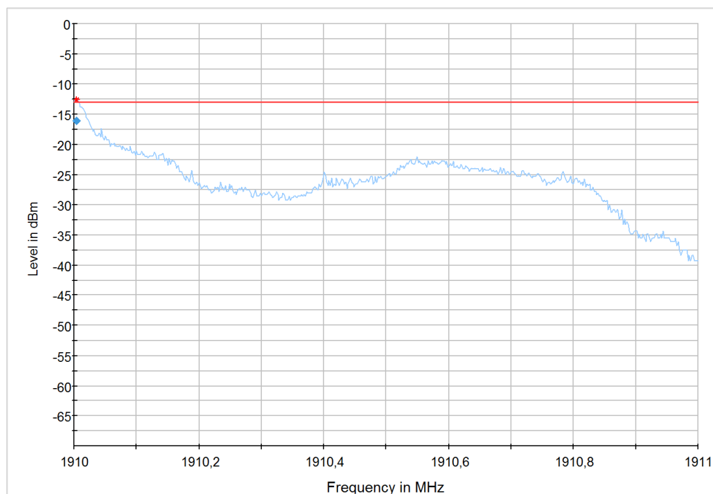
Diagram 8: 9.214b_LTE2_CH19193_BW1,4_RB1high_16QAM
