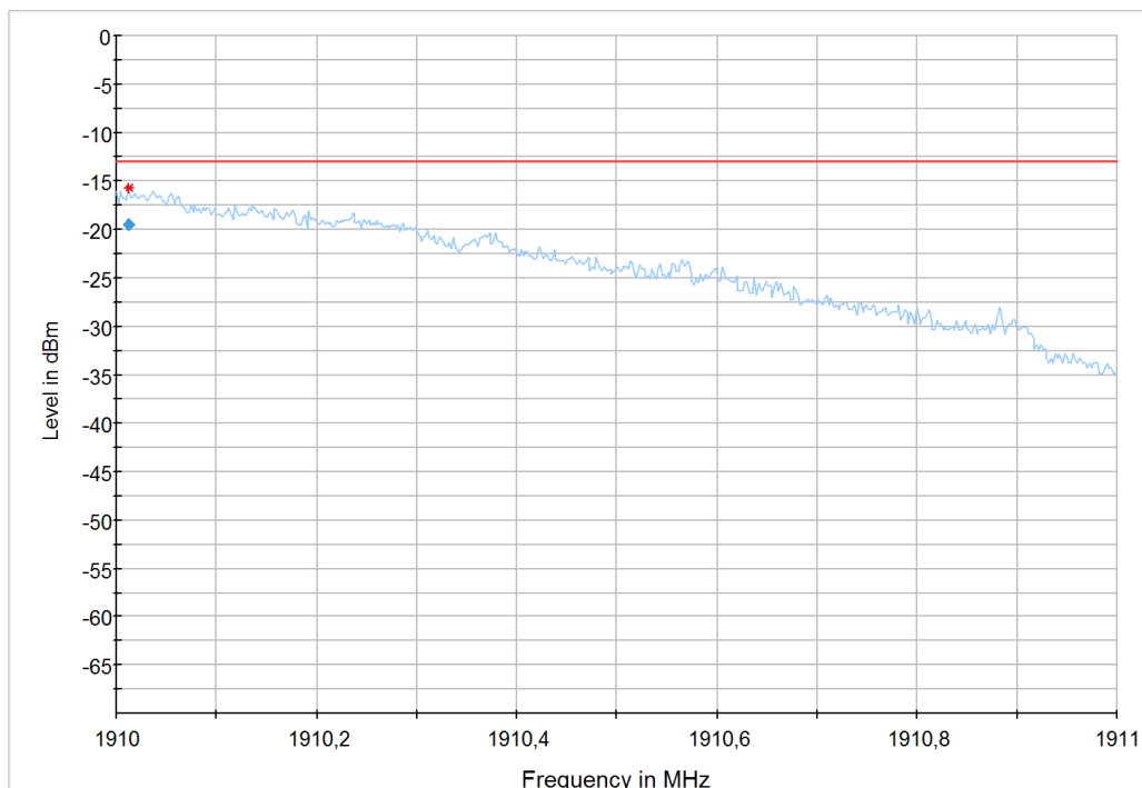
Diagram 5: 9.213a_LTE2_CH19193_BW1,4_RB6high_QPSK
