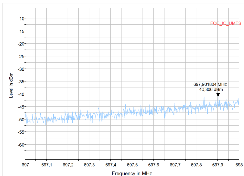
Diagram 69: 9.1203b_LTE12_CH23025_BW3_RB1low_16QAM
