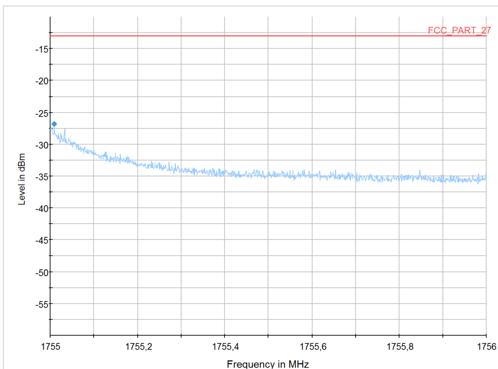
Diagram 28: 9.416b_LTE4_Ch20385_RB15high_BW3MHz_16QAM
