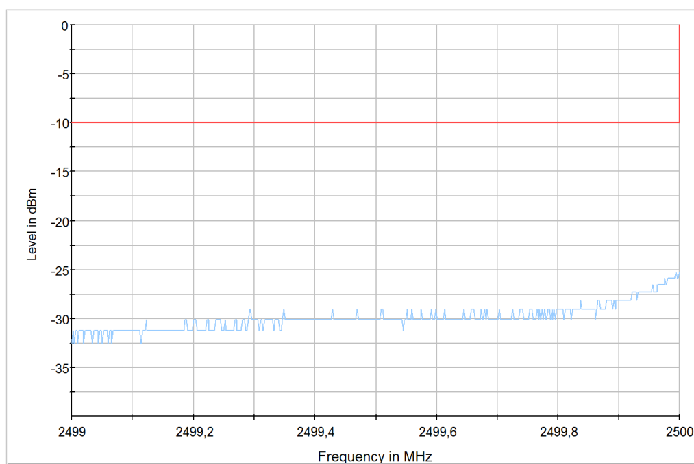
Diagram 45: 9.702a_SW2_LTE7_CH20775_BW5_RB25_LOW_QPSK
