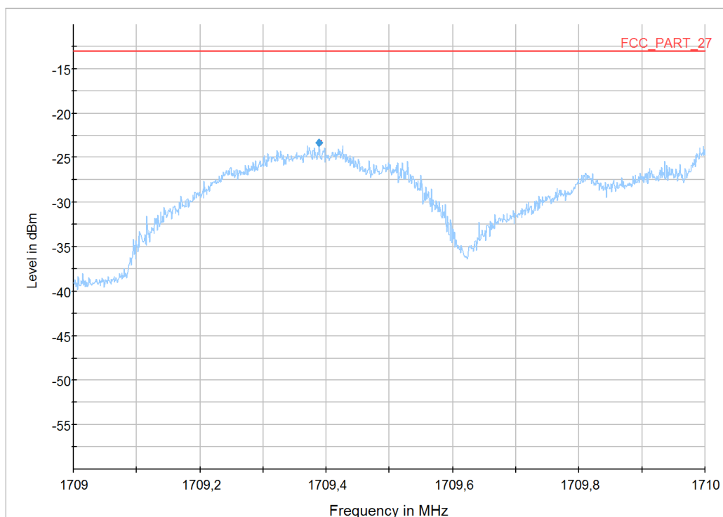
Diagram 13: 9.401a_LTE4_Ch19957_RB1low_BW1,4MHz_QPSK
