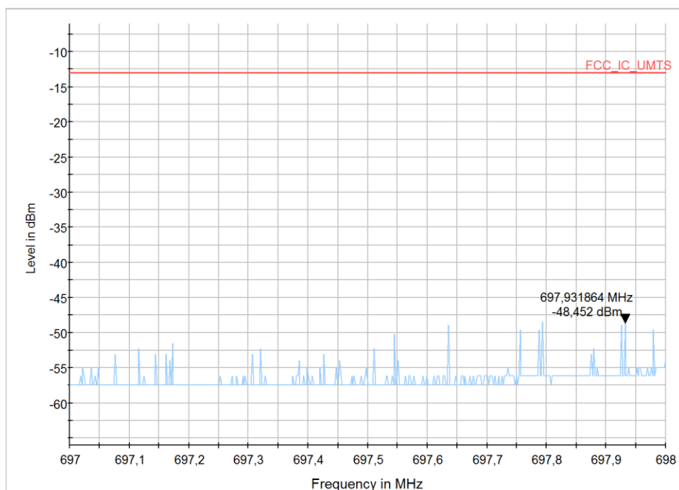
Diagram 68: 9.1203a_LTE12_CH23025_BW3_RB1low_QPSK
