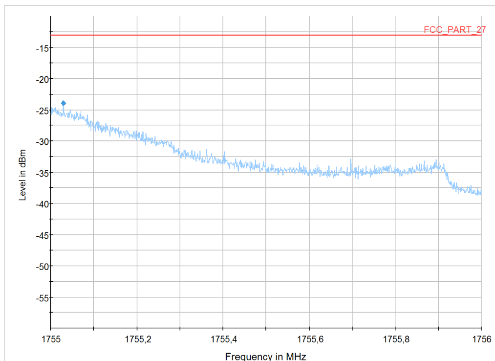
Diagram 23: 9.414a_LTE4_Ch20393_RB6high_BW1,4MHz_QPSK
