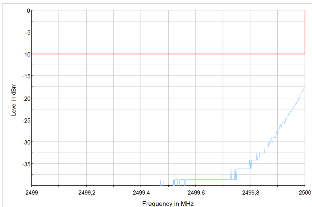
Diagram 39: 9.701a_SW2_LTE7_CH20775_BW5_RB1_LOW_QPSK
