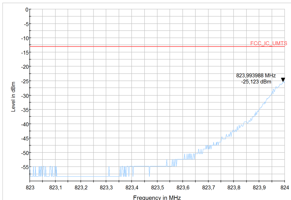
Diagram 29: 9.503a_LTE5_Ch20415_RB1Low_BW3MHz_QPSK
