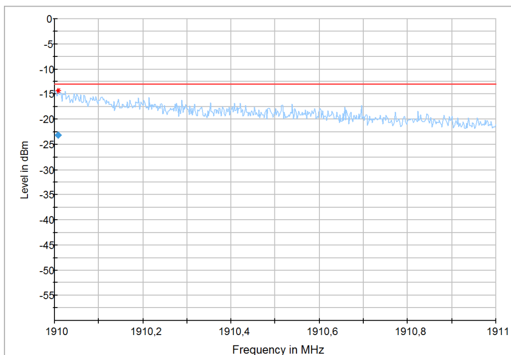
Diagram 11: 9.216a_LTE2_CH19185_BW3_RB15high_QPSK
