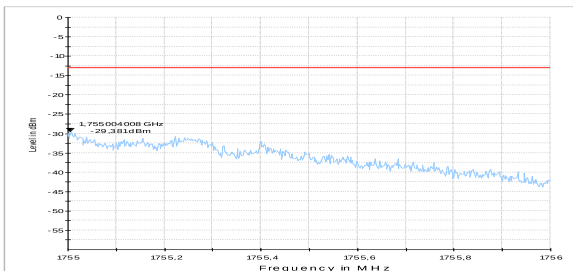
Diagram 9.43b_Ch20393_BW_1.4MHz_6RBs_16QAM
