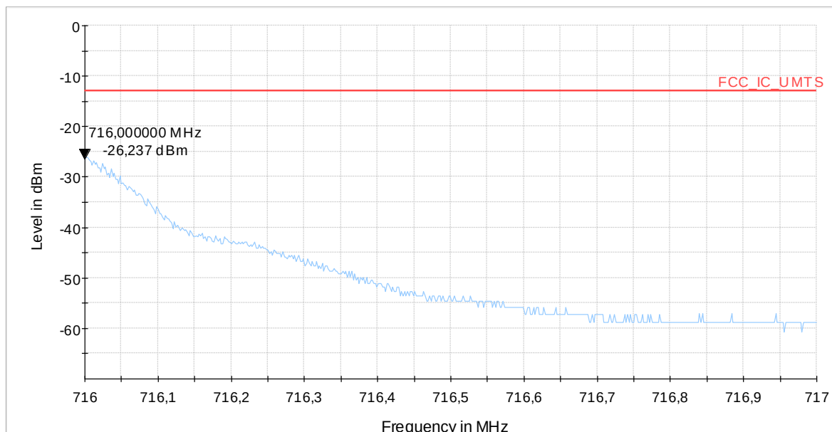
Diagram 9.1703a_Ch23825_BW_5MHz_1RBhigh_QPSK
