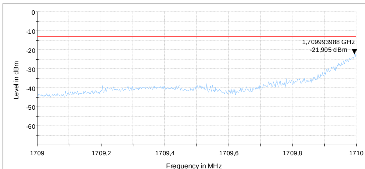
Diagram 9.40a_Ch19957_BW_1.4MHz_1RBlow_QPSK
