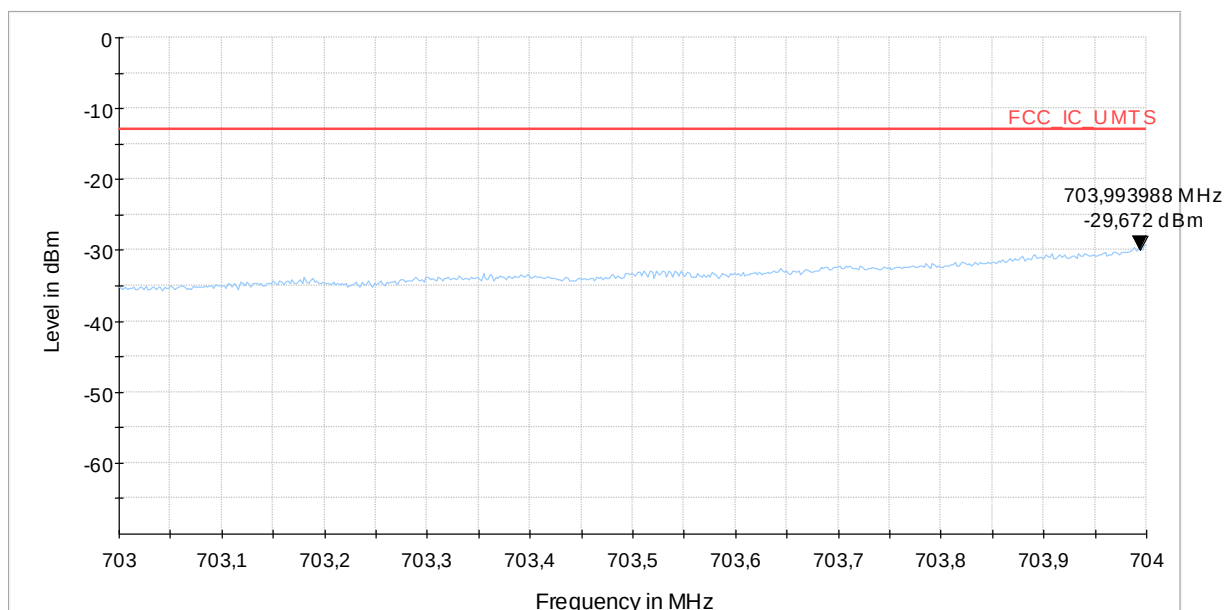
Diagram 9.1702a_Ch23755_BW_5MHz_25RBS_QPSK
