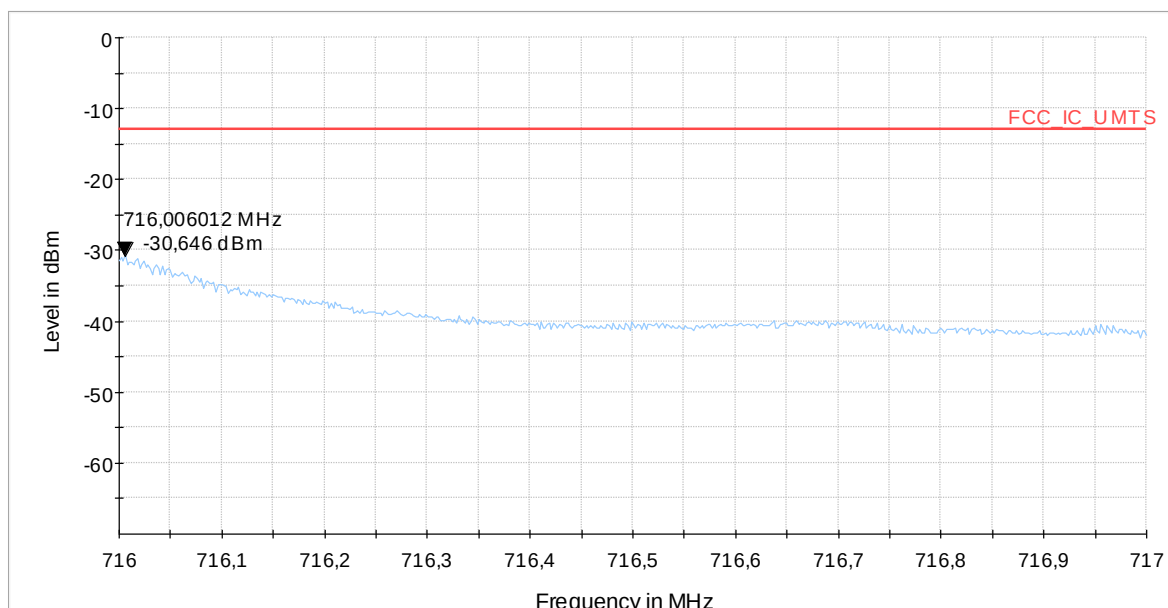
Diagram 9.1704a_Ch23825_BW_5MHz_25RBS_QPSK
