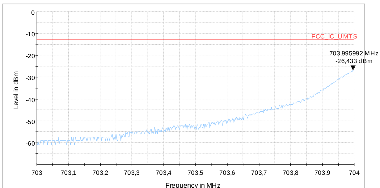
Diagram 9.1701b_Ch23755_BW_5MHz_1RBlow_16QAM
