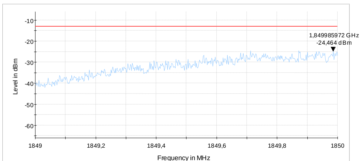
Diagram 9.21b_Ch18607BW_1.4MHz_6RBs_16QAM
