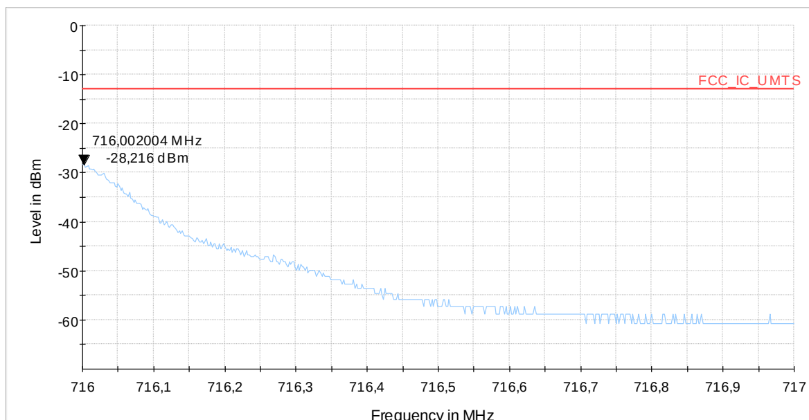
Diagram 9.1703b_Ch23825_BW_5MHz_1RBhigh_16QAM
