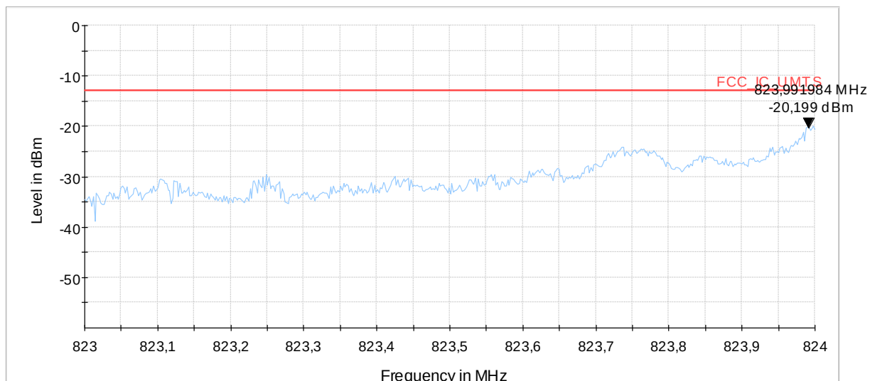
Diagram 9.501a_Ch20407_BW_1.4MHz_6RBs_QPSK
