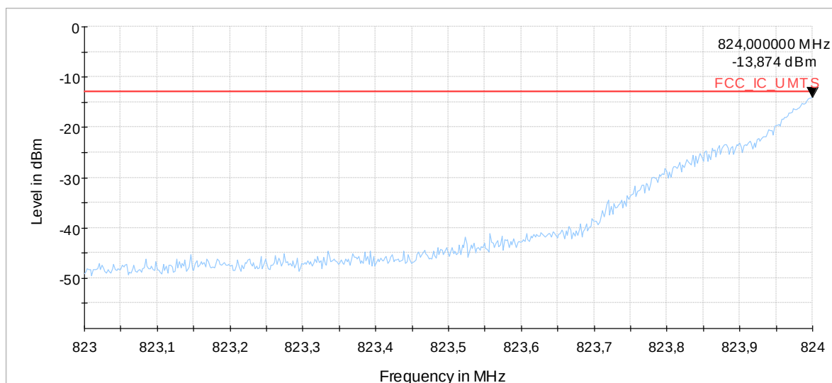
Diagram 9.500a_Ch20407_BW_1.4MHz_1RBlow_QPSK
