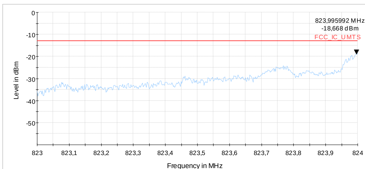
Diagram 9.501b_Ch20407_BW_1.4MHz_6RBs_16QAM
