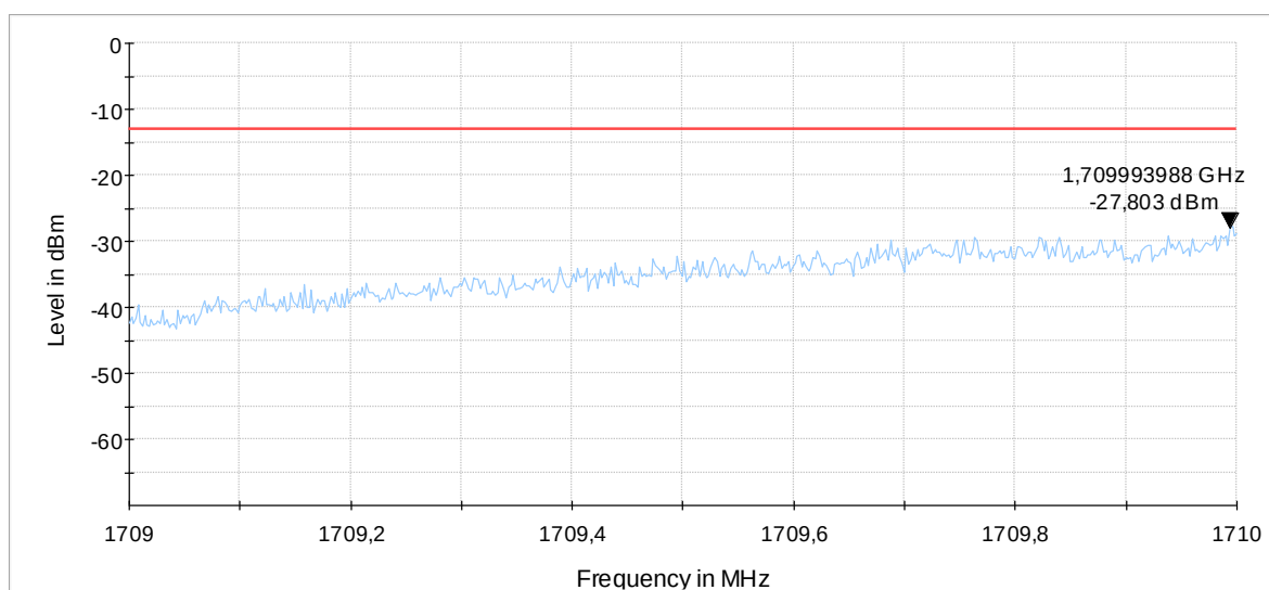
Diagram 9.41b_Ch19957_BW_1.4MHz_6RBs_16QAM
