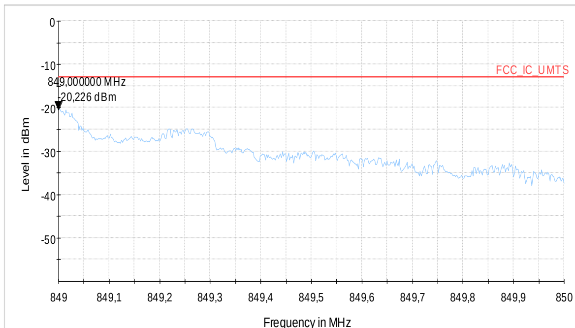
Diagram 9.503a_Ch20643_BW_1.4MHz_6RBs_QPSK
