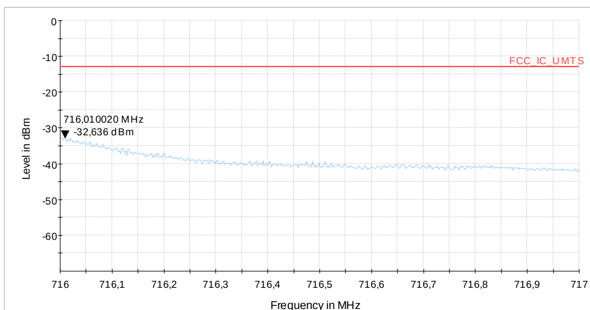
Diagram 9.1704b_Ch23825_BW_5MHz_25RBs_16QAM
