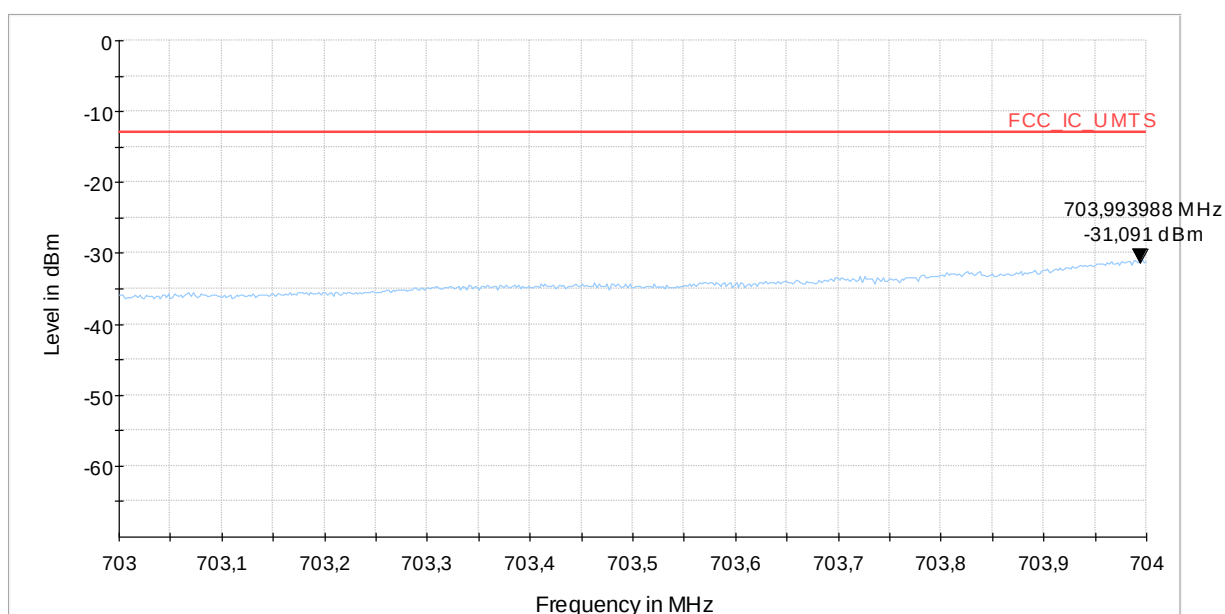
Diagram 9.1702b_Ch23755_BW_5MHz_25RBs_16QAM
