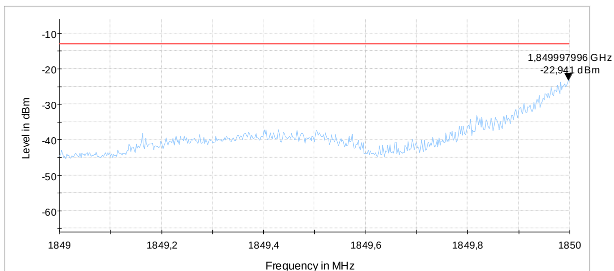
Diagram 9.20b_Ch18607BW_1.4MHz_1RBlow_16QAM
