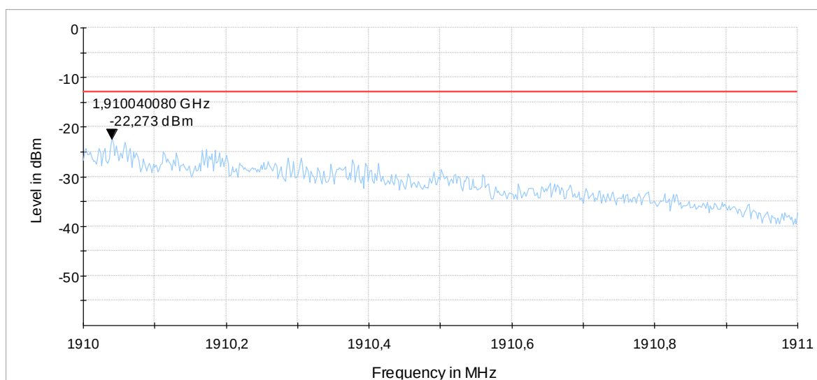
Diagram 9.23b_Ch19193_BW_1.4MHz_6RBs_16QAM
