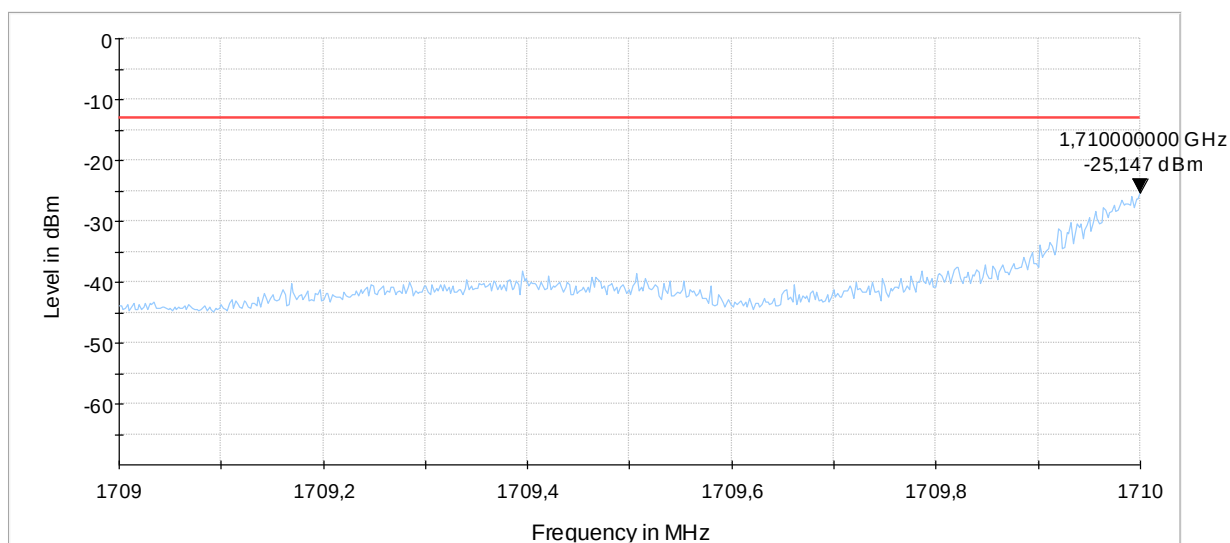
Diagram 9.40b_Ch19957_BW_1.4MHz_1RBlow_16QAM
