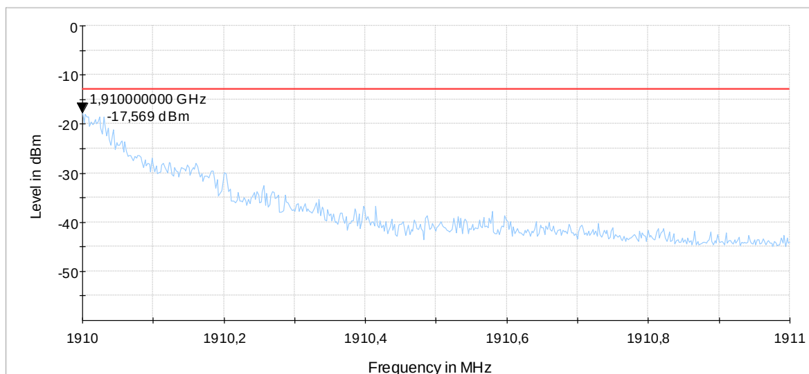
Diagram 9.22a_Ch19193_BW_1.4MHz_1RBhigh_QPSK
