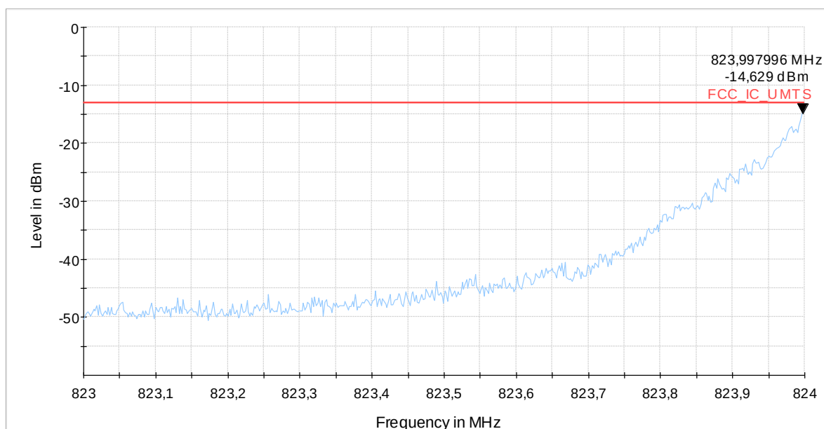
Diagram 9.500b_Ch20407_BW_1.4MHz_1RBlow_16QAM
