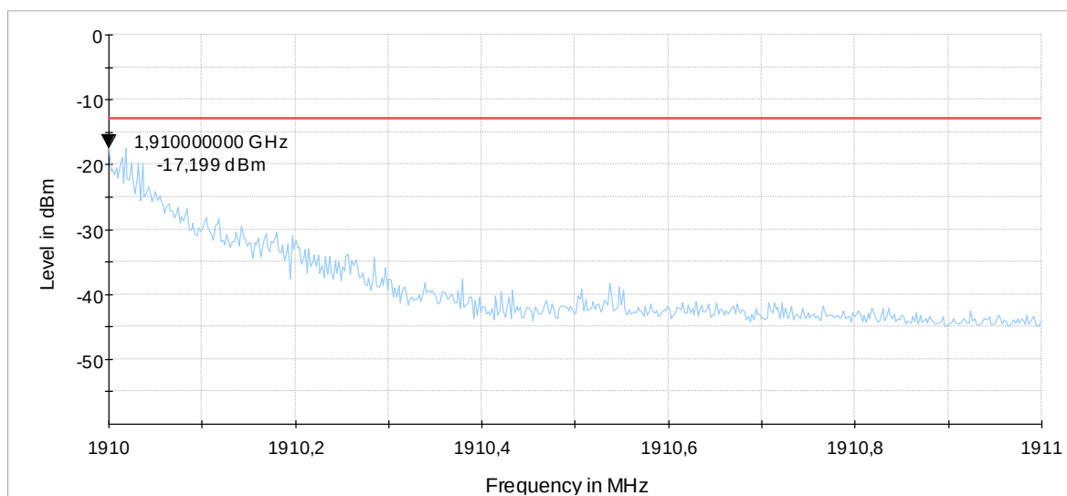
Diagram 9.22b_Ch19193_BW_1.4MHz_1RBhigh_16QAM
