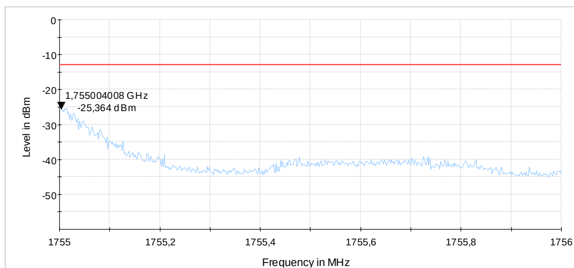
Diagram 9.42b_Ch20393_BW_1.4MHz_1RBhigh_16QAM
