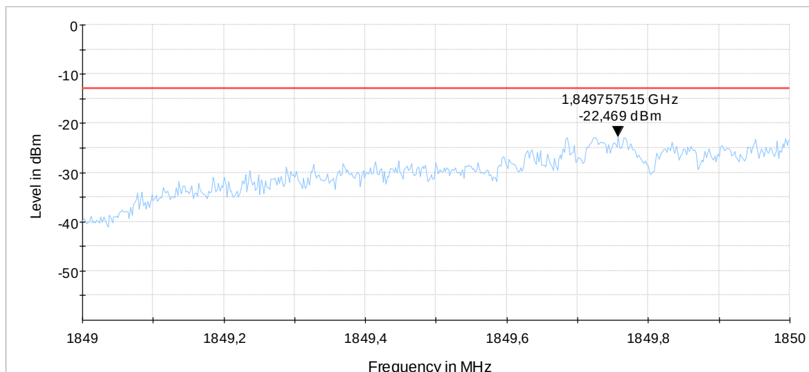
Diagram 9.21a_Ch18607BW_1.4MHz_6RBs_QPSK
