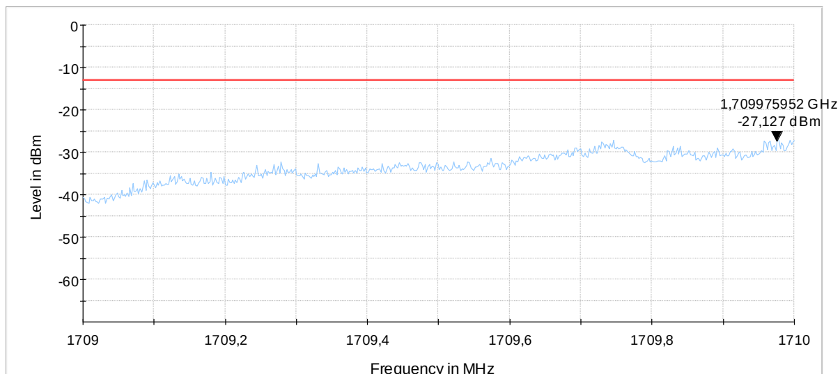
Diagram 9.41a_Ch19957_BW_1.4MHz_6RBs_QPSK
