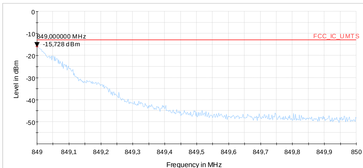
Diagram 9.502a_Ch20643_BW_1.4MHz_1RBhigh_QPSK
