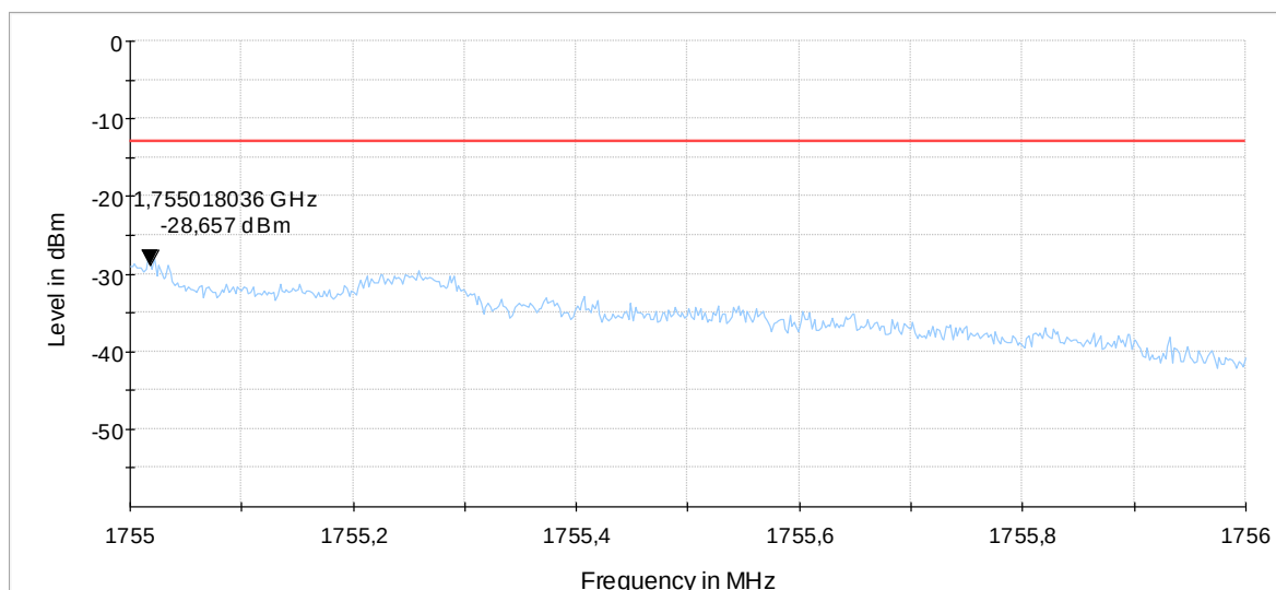
Diagram 9.43a_Ch20393_BW_1.4MHz_6RBs_QPSK
