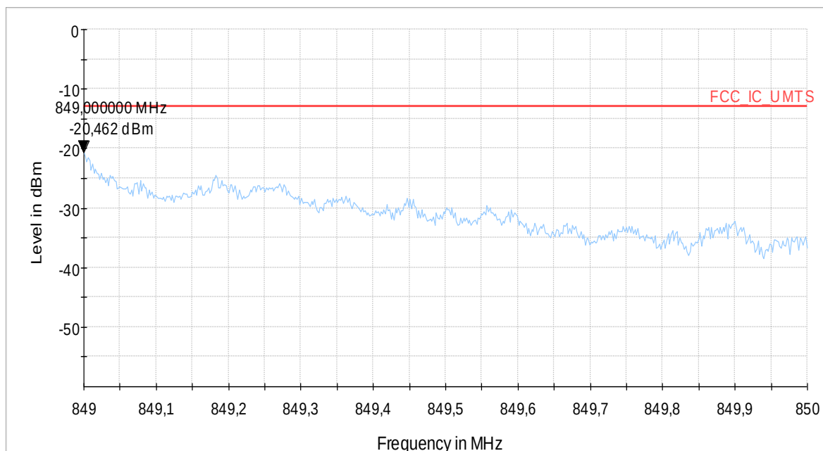
Diagram 9.503b_Ch20643_BW_1.4MHz_6RBs_16QAM
