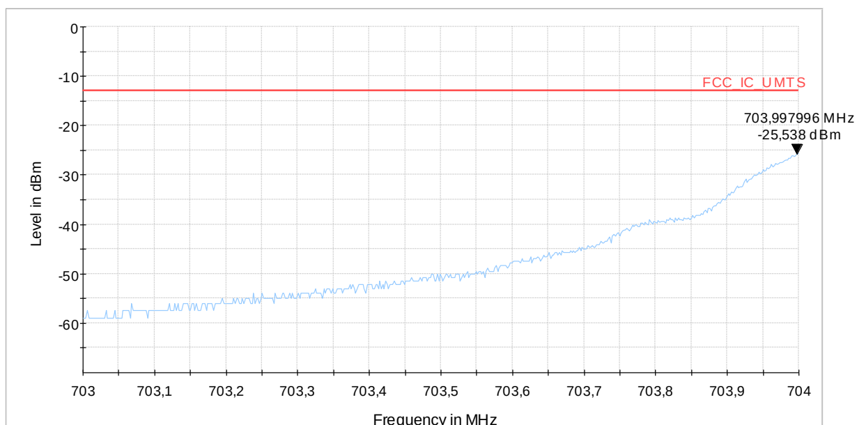
Diagram 9.1701a_Ch23755_BW_5MHz_1RBlow_QPSK
