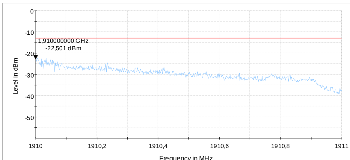
Diagram 9.23a_Ch19193_BW_1.4MHz_6RBs_QPSK
