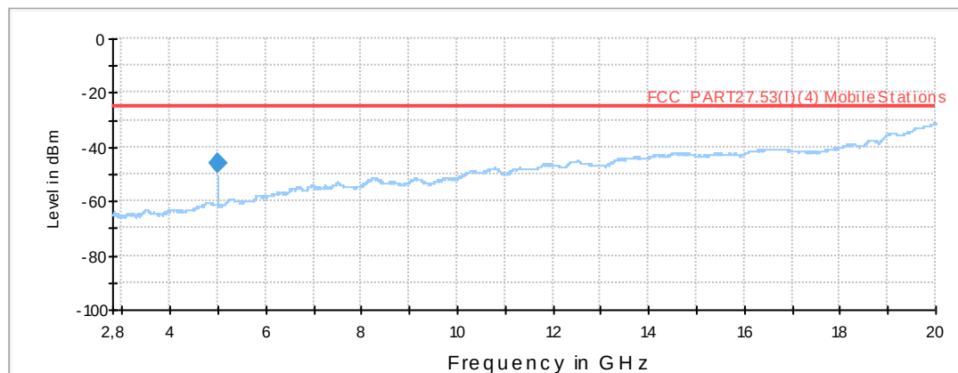
030421_Sweep2_FCC_Part27_LTE7_TX_all_channels_2.8-20GHz_no_kipf
