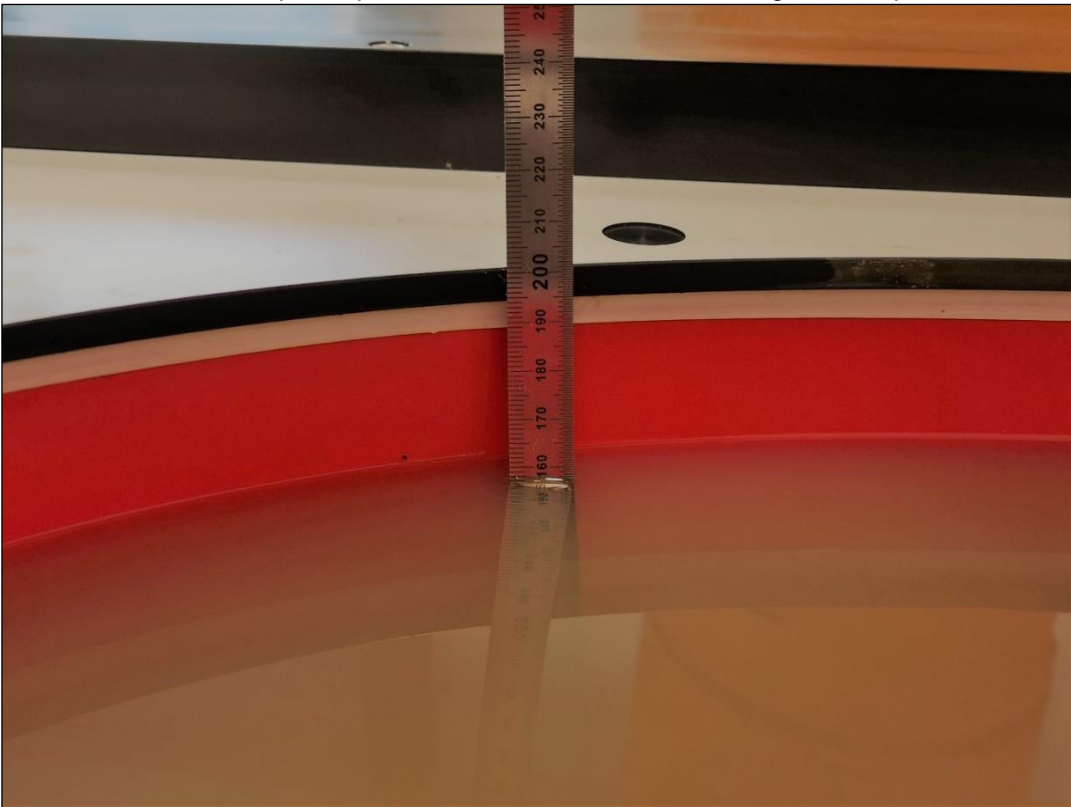
Photo 8: Liquid depth HBBL600-10000MHz Simulating Head Liquid
