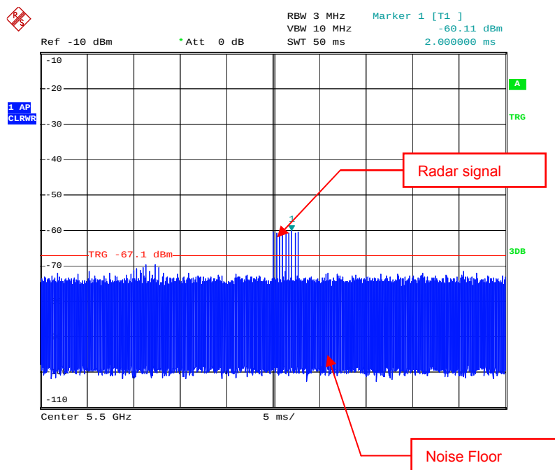
Single Burst of Radar Signal 5
