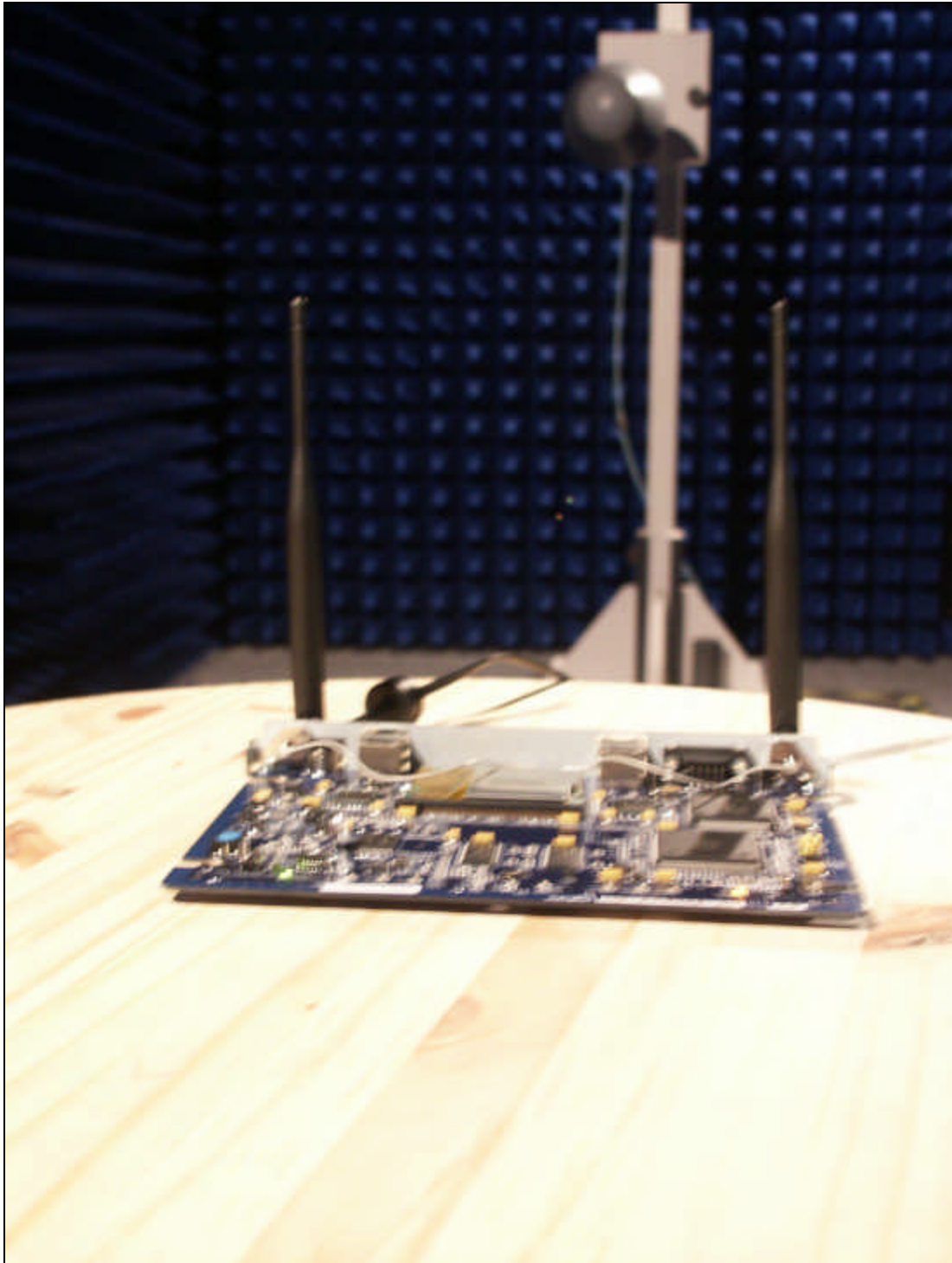
Radiated emission
