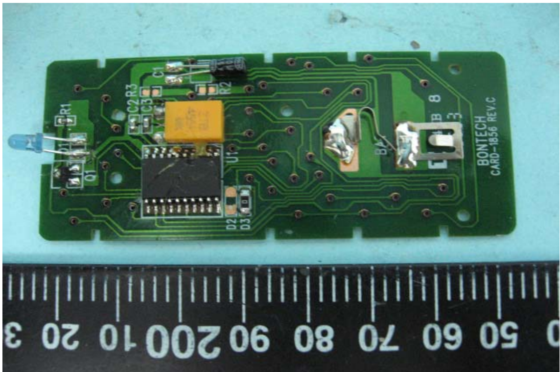
Solder View of Remoter control's PCB
