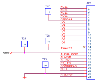
ACE87152-0240 (FPC Connector 24 pin)
