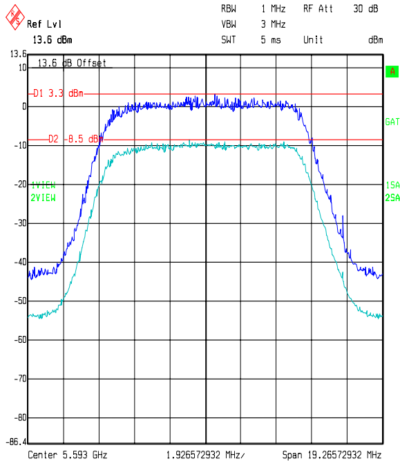
Title: Peak Excursion for Motorola JN: 48672JD02 Comment A: QPSK Mid Channel PORT H Date: 12.OCT.2006 13:37:40
