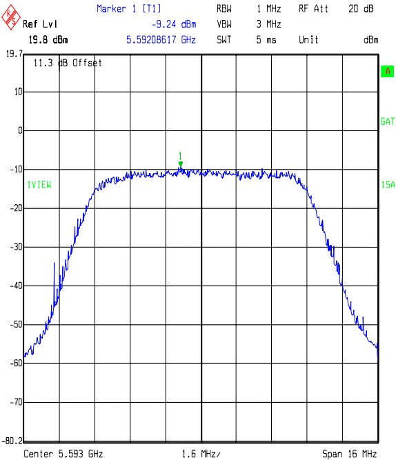
Title: Power Spectral Density for Motorola JN: 48672 Comment A: Middle Channel -BPSK Date: 18.OCT.2006 14:40:58
