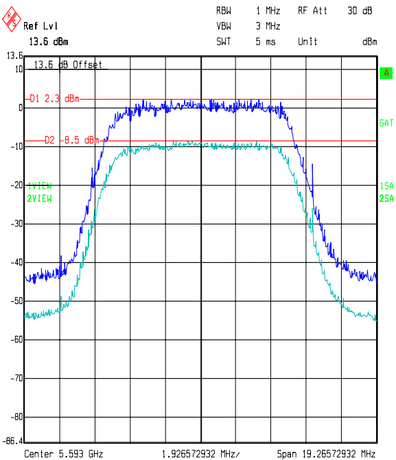
Title: Peak Excursion for Motorola JN: 48672JD02 Comment A: ACQ Mid Channel PORT H Date: 12.OCT.2006 14:40:37
