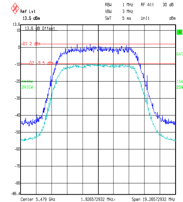
Title: Peak Excursion for Motorola JN: 48672JD02 Comment A: ACQ Bot Channel PORT H Date: 12.OCT.2006 14:36:42
