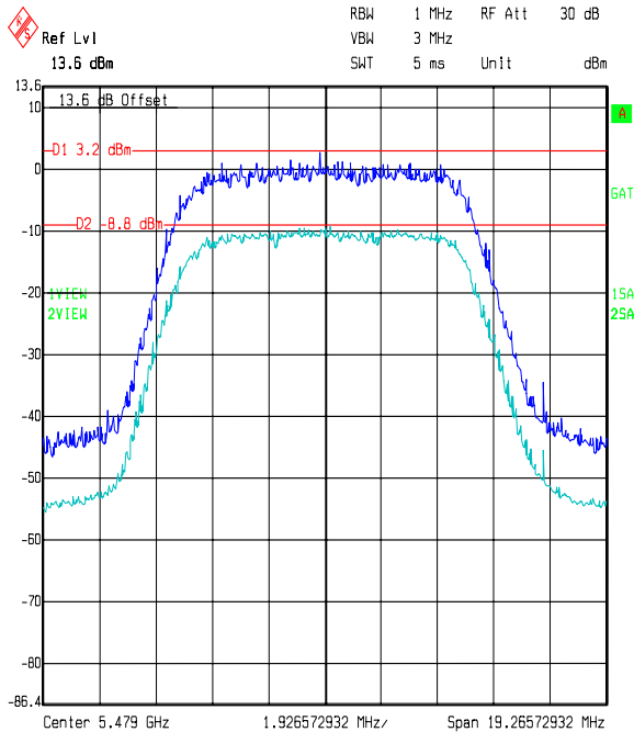
Title: Peak Excursion for Motorola JN: 48672JD02 Comment A: BPSK Bot Channel PORT H Date: 12.OCT.2006 13:45:34
