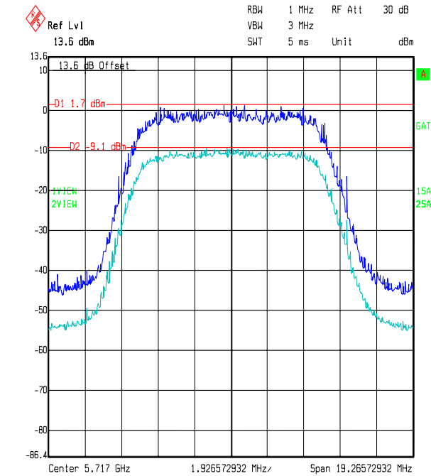
Title: Peak Excursion for Motorola JN: 48672JD02 Comment A: ACQ Top Channel PORT H Date: 12.OCT.2006 14:44:57
