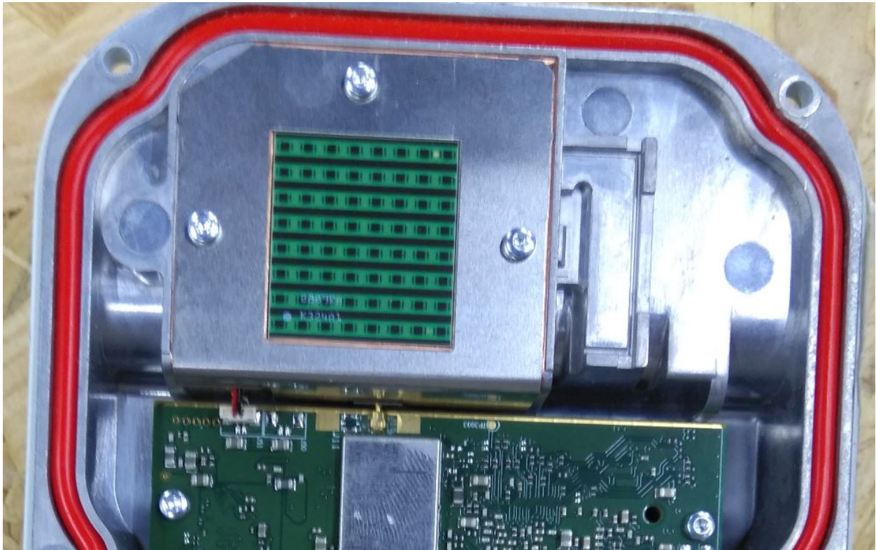
V1000 SSPXA-001326 SWL-QD46 RF Tile Installed View
