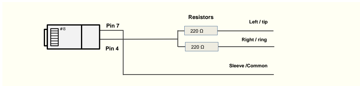
Figure 21 Alignment Tone Cable
