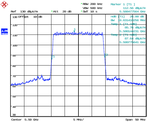
QPSK 5590 MHz
