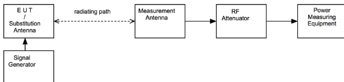
Figure v Test Setup
