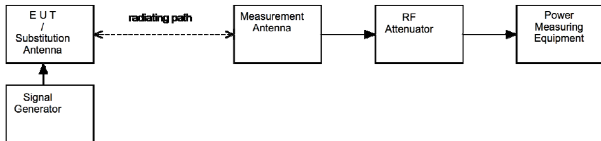
Figure v Test Setup
