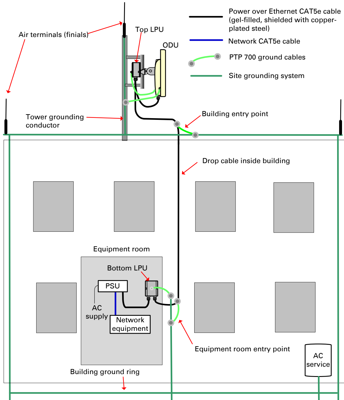
Figure 37 Roof installation
