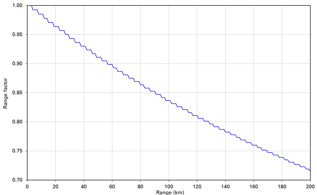
Figure 104 Range adjustment for PTP 700, adaptive, optimization IP, bandwidth 10 MHz
