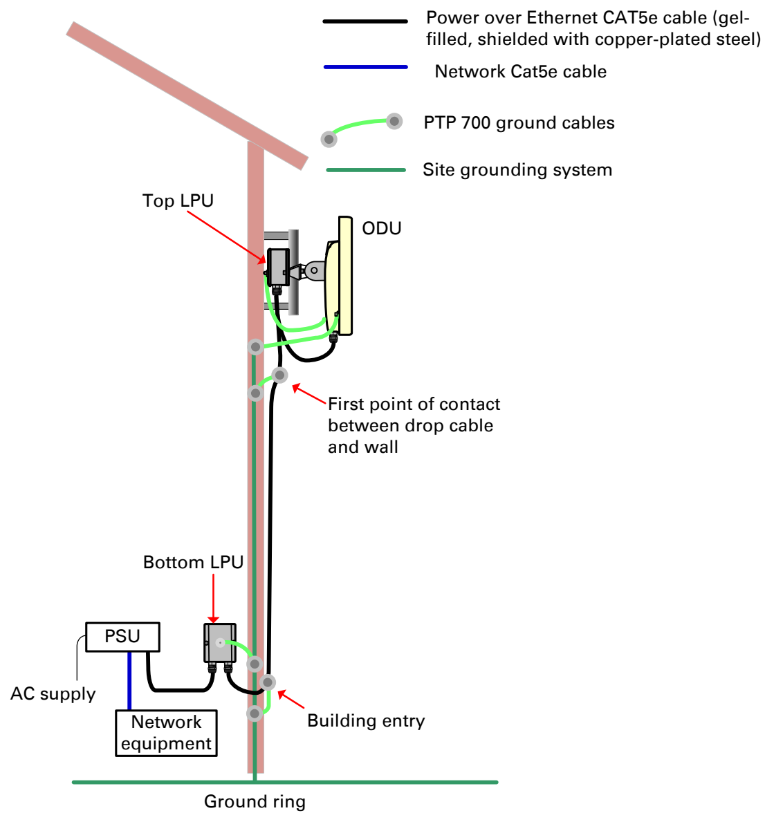
Figure 36 Wall installation
