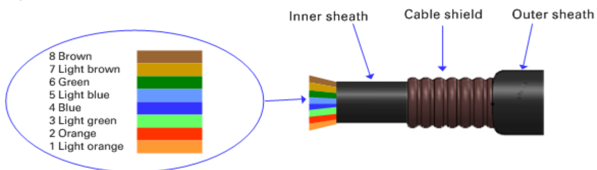
Figure 20 Outdoor drop cable
