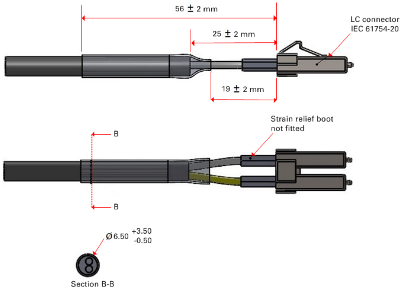
Figure 27 Optical optic cable and connector specification
