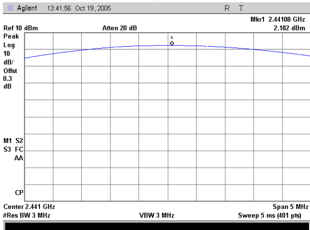
Middle Channel (operating at 2441 MHz)
