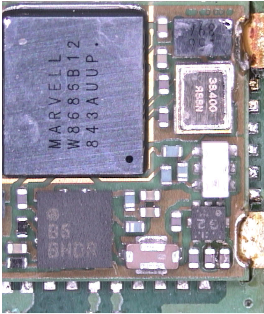
Figure 3 Internal view of Murata hybrid with cover removed.
