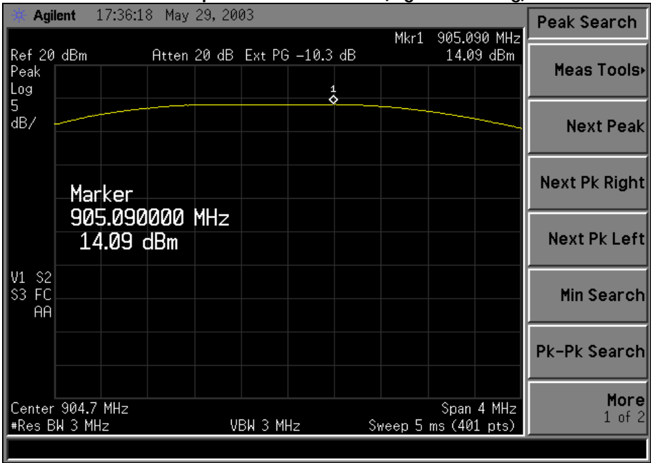
Signature Scan of Conducted RF Power measurements, Table-Top Unit, Low Channel (highest reading)
