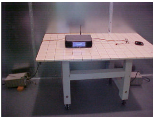
Setup for the Conducted Emissions Test on the Table-Top Unit:
