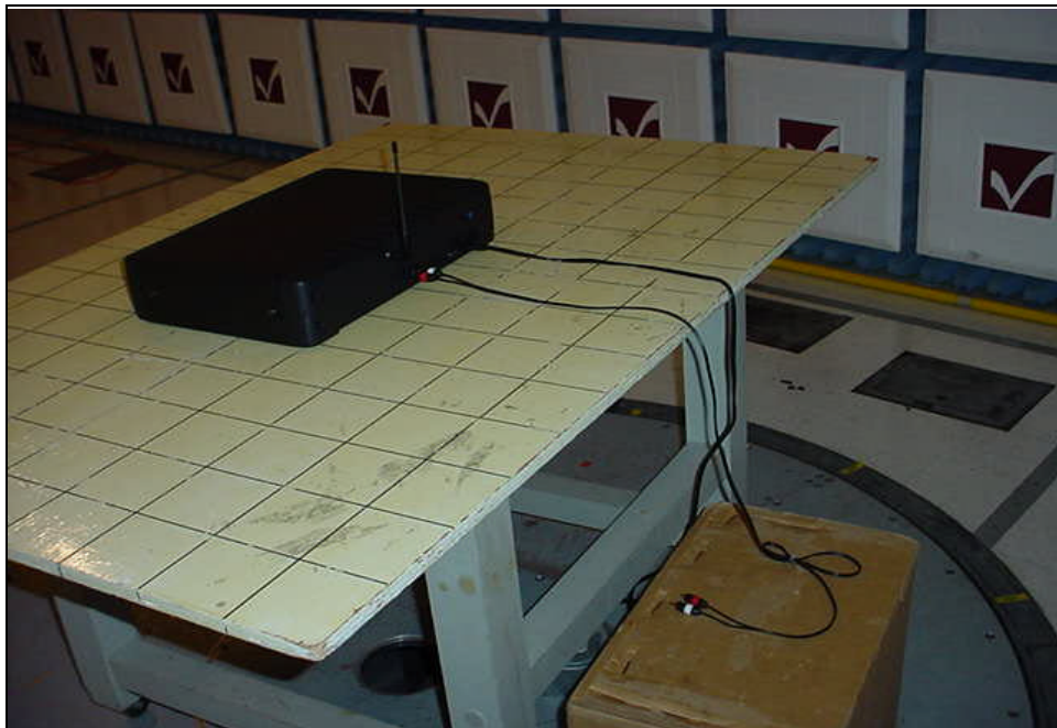
View of populated ports in rear of EUT
