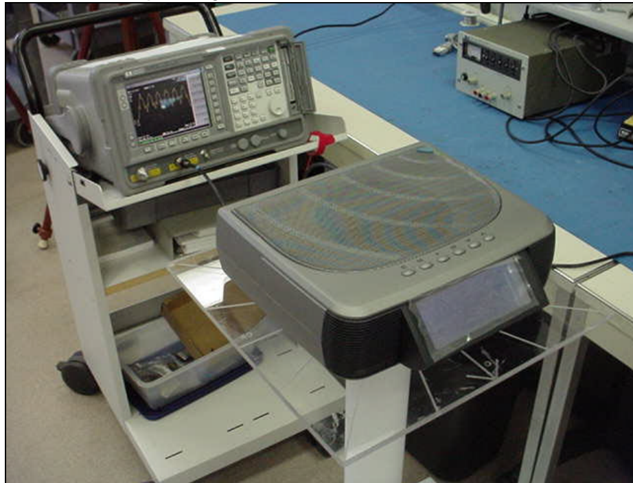
View of Test Setup During the Conducted RF measurements, Table-Top Unit
