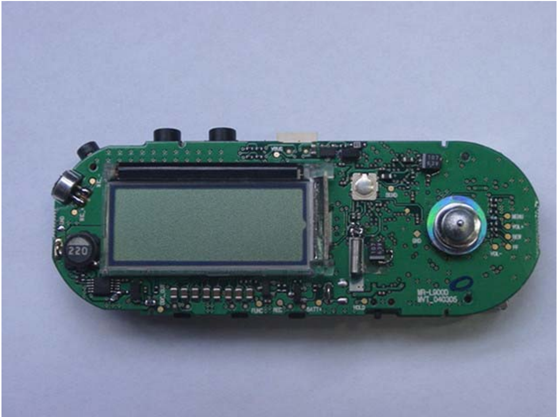
<FULL INNER SIDE OF EUT>
