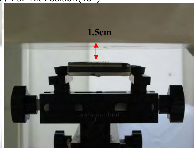
Fig.7 Body worn- EUT Back to flat phantom and distance between flat phantom and mobile phone is 1.5 cm
