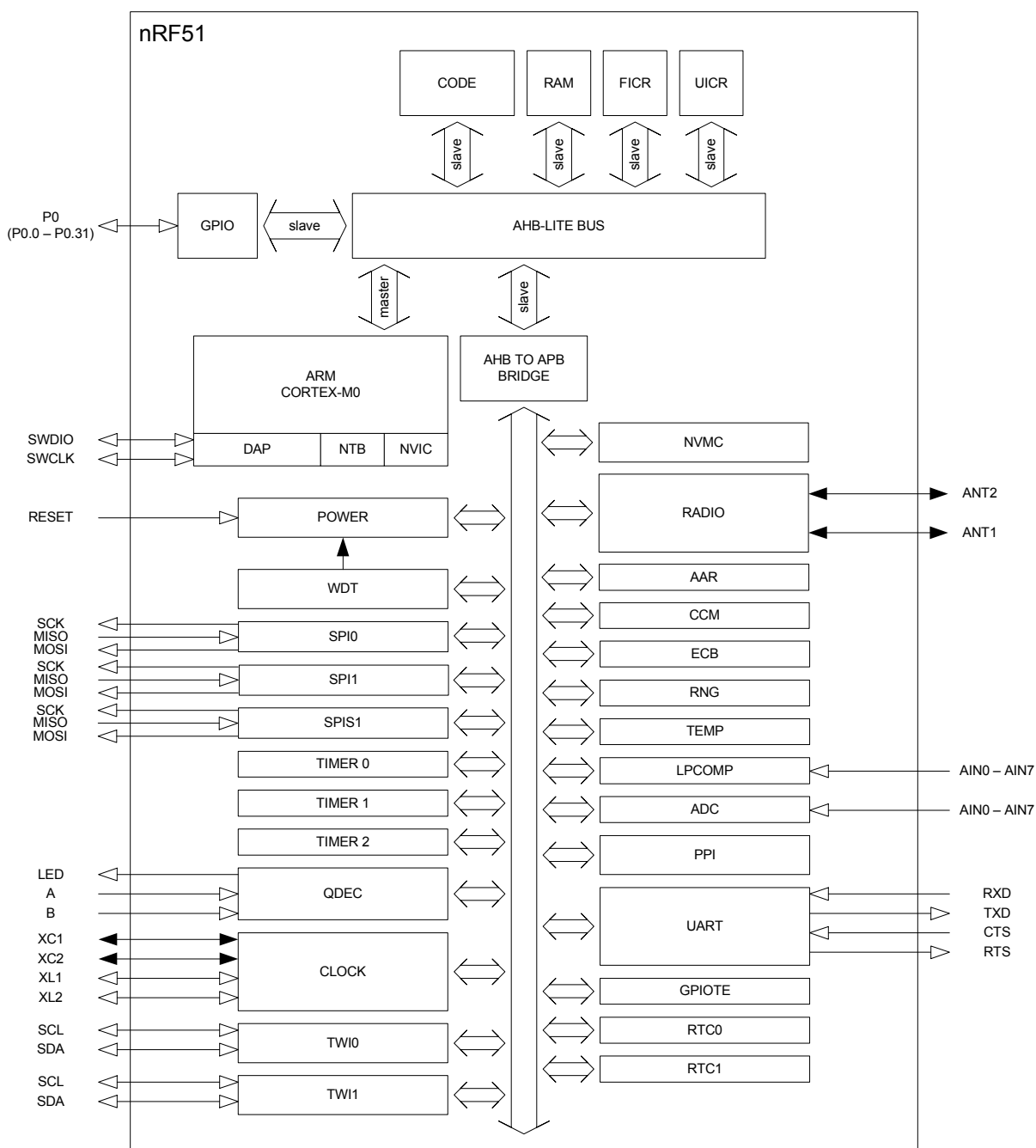
Figure 1 Block diagram
