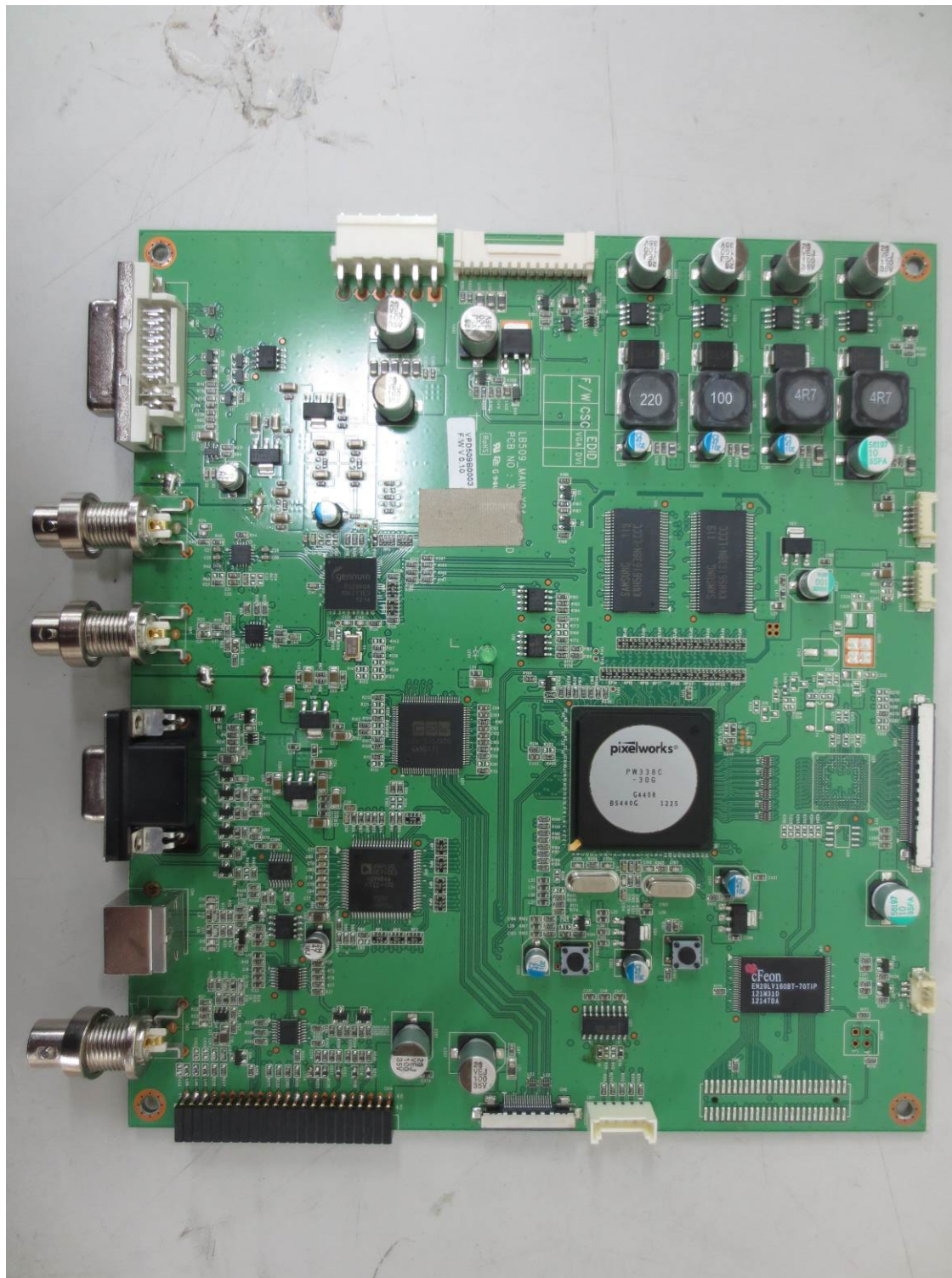
Main-Board front
