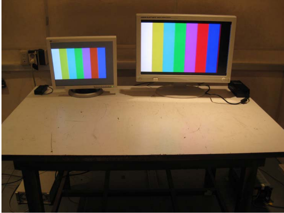
Conducted Emission Test Setup, SDI In, Out Mode, side
