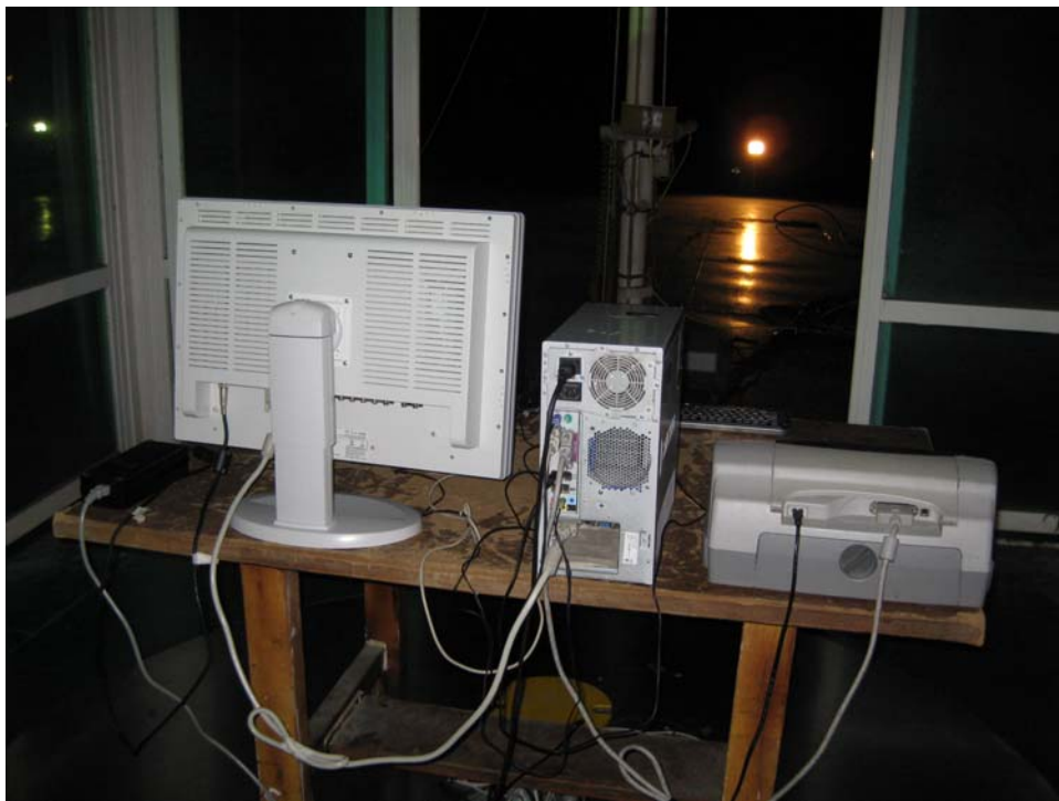
Radiated emission test setup, DVI Mode, 1GHz to 2GHz, rear
