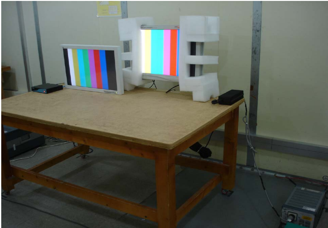
Figure 2. Test Setup for Conducted Emissions (SDI Mode)
