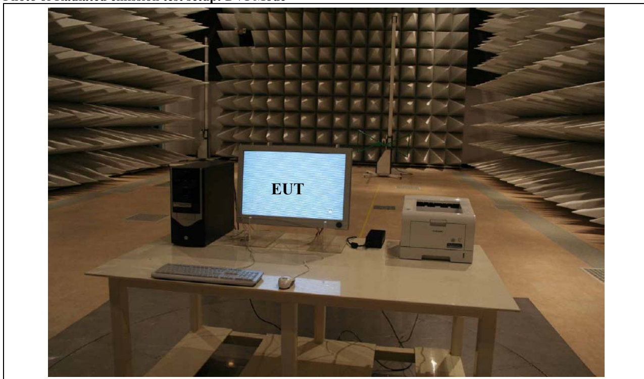
Photo of Radiated emission test setup: DVI Mode
