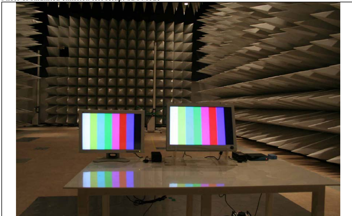
Figure 4 Photo of Radiated emission test setup: SDI Mode
