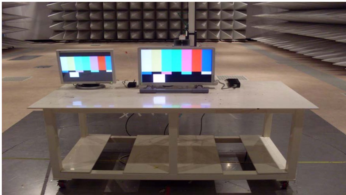
Figure 9, Radiated emission test setup for Test Configuration 2
