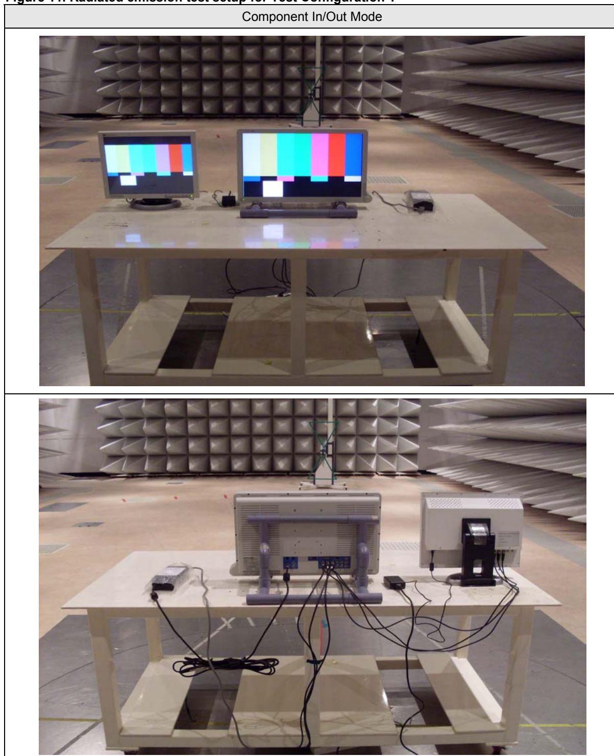
Figure 11. Radiated emission test setup for Test Configuration 1
