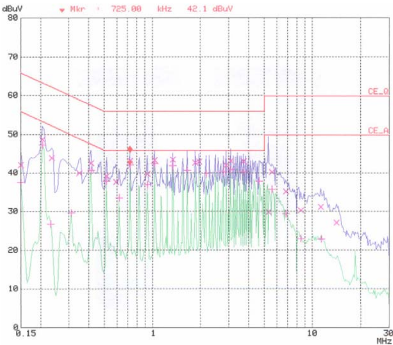
< Hot line >
