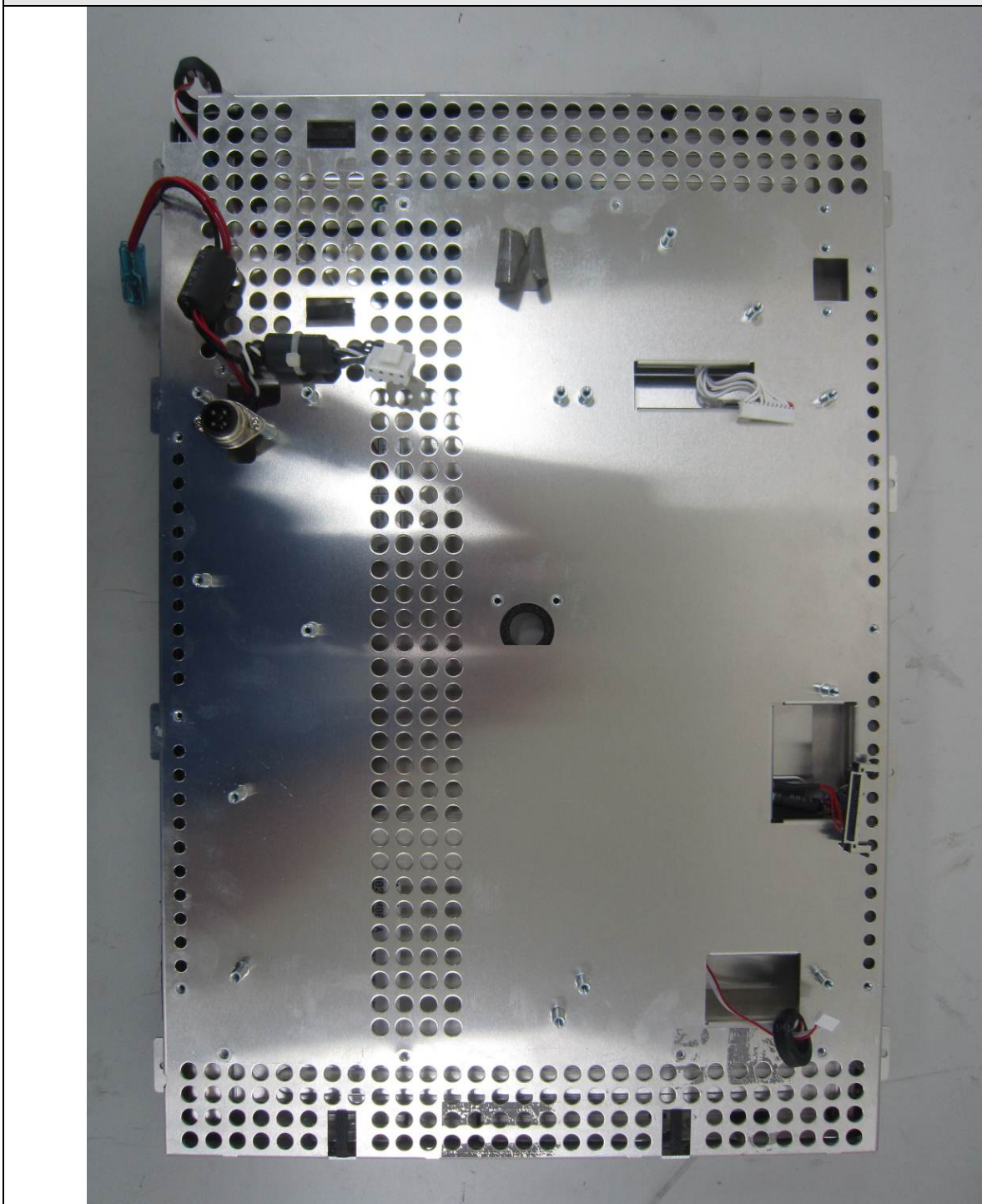
LCD Panel Rear View
