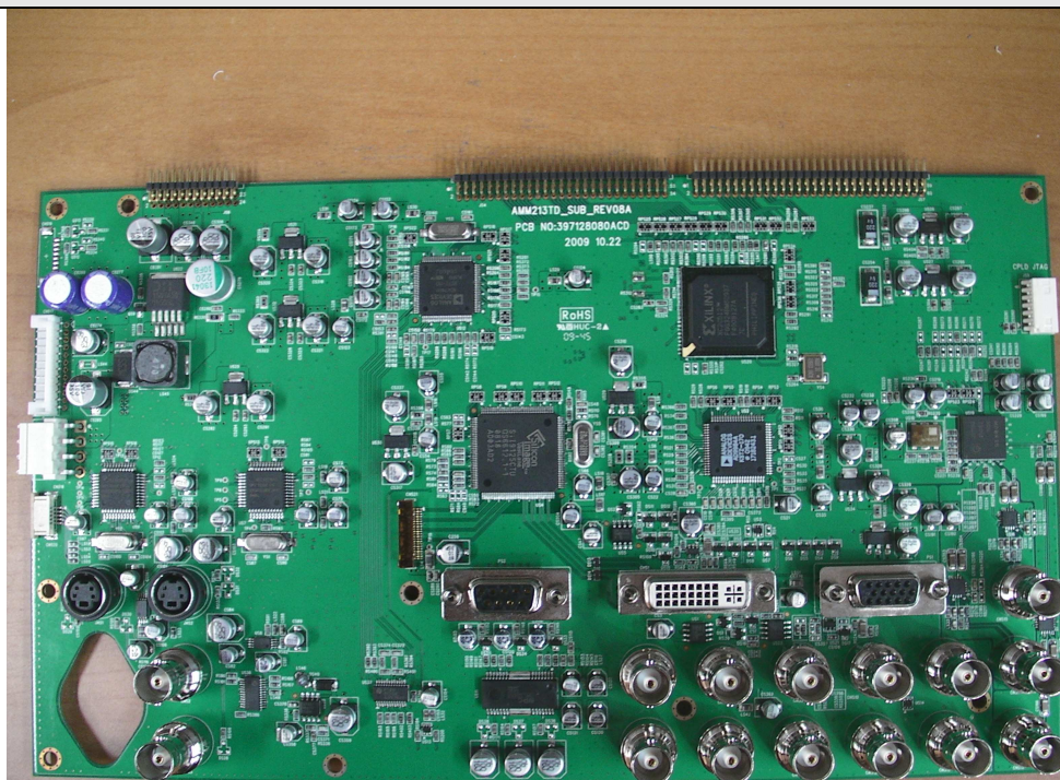
SUB Board
