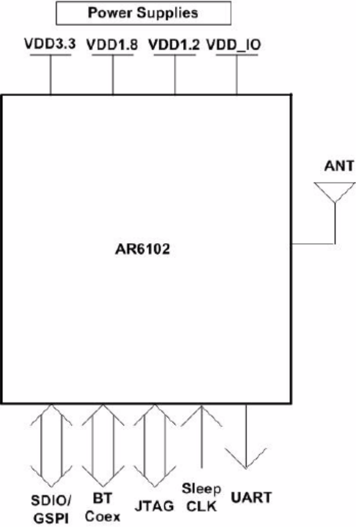
Atheros AR6102 Block Diagram
