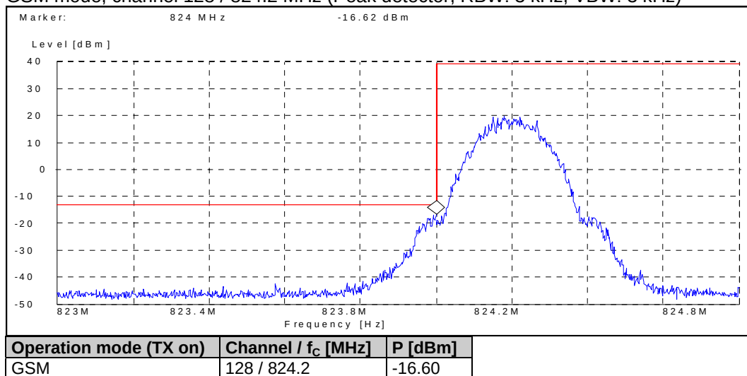
GSM mode, channel 128 / 824.2 MHz (Peak detector, RBW: 3 kHz, VBW: 3 kHz)
