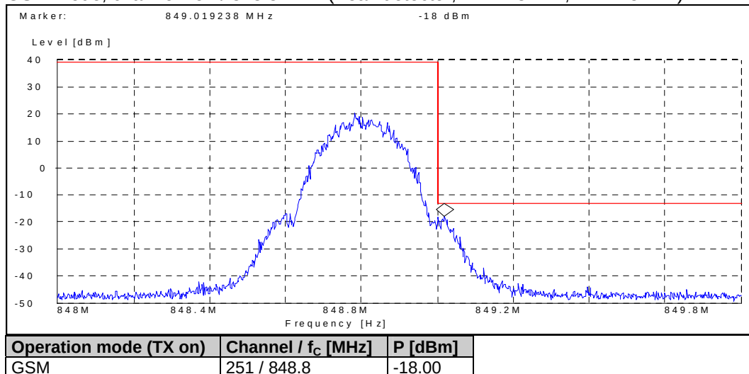
GSM mode, channel 251 / 848.8 MHz (Peak detector, RBW: 3 kHz, VBW: 3 kHz)
