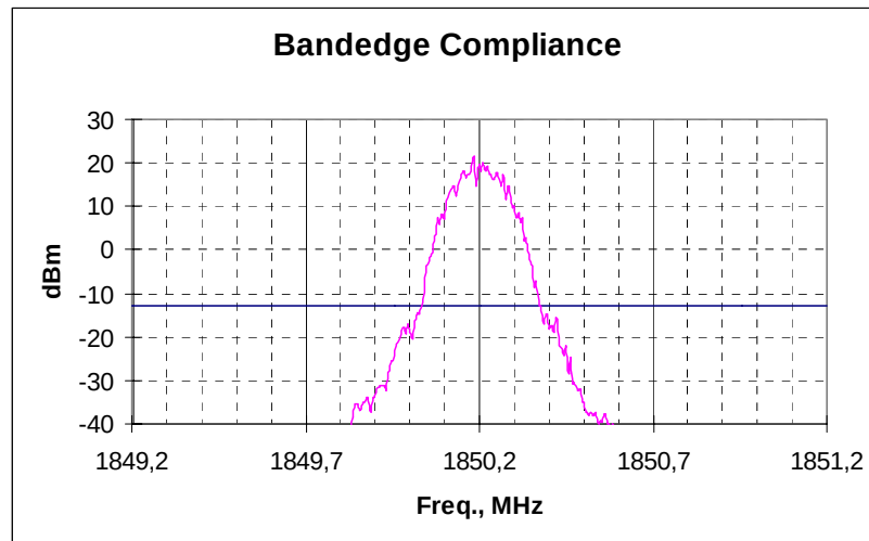
Picture 5. Lower bandedge, channel 512, RBw 3KHz VBw 3KHz
