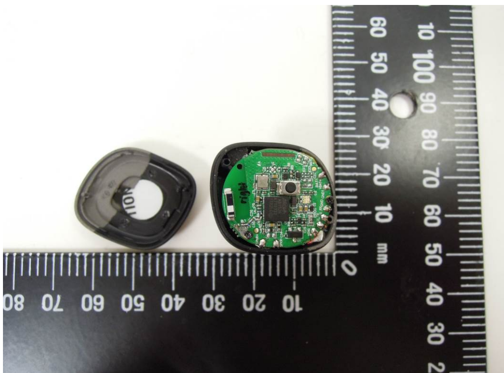
Open View of EUT - 1 (Right)
