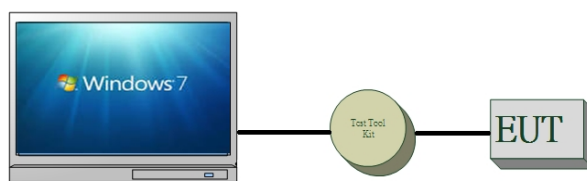
Fig.2-2 Conducted Emission (Antenna Port) Configuration
