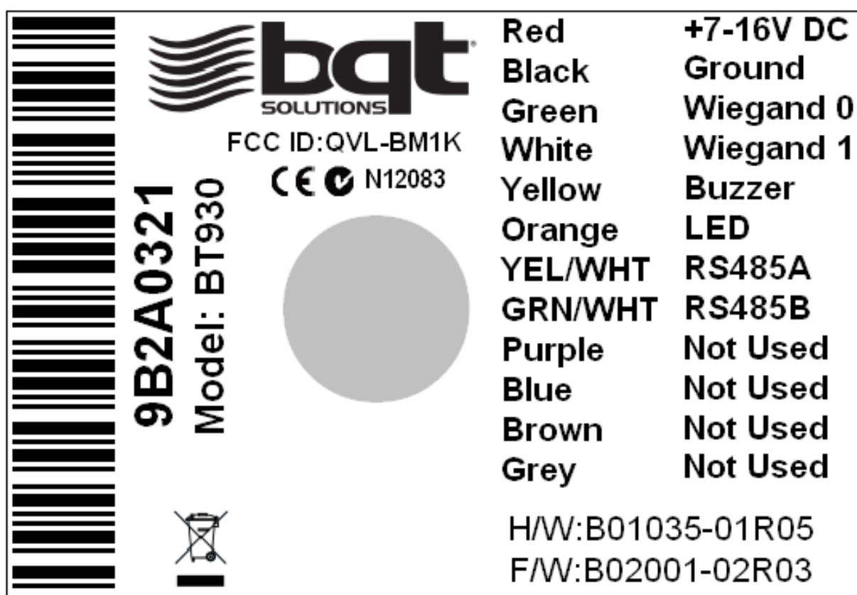
BT930 Label
