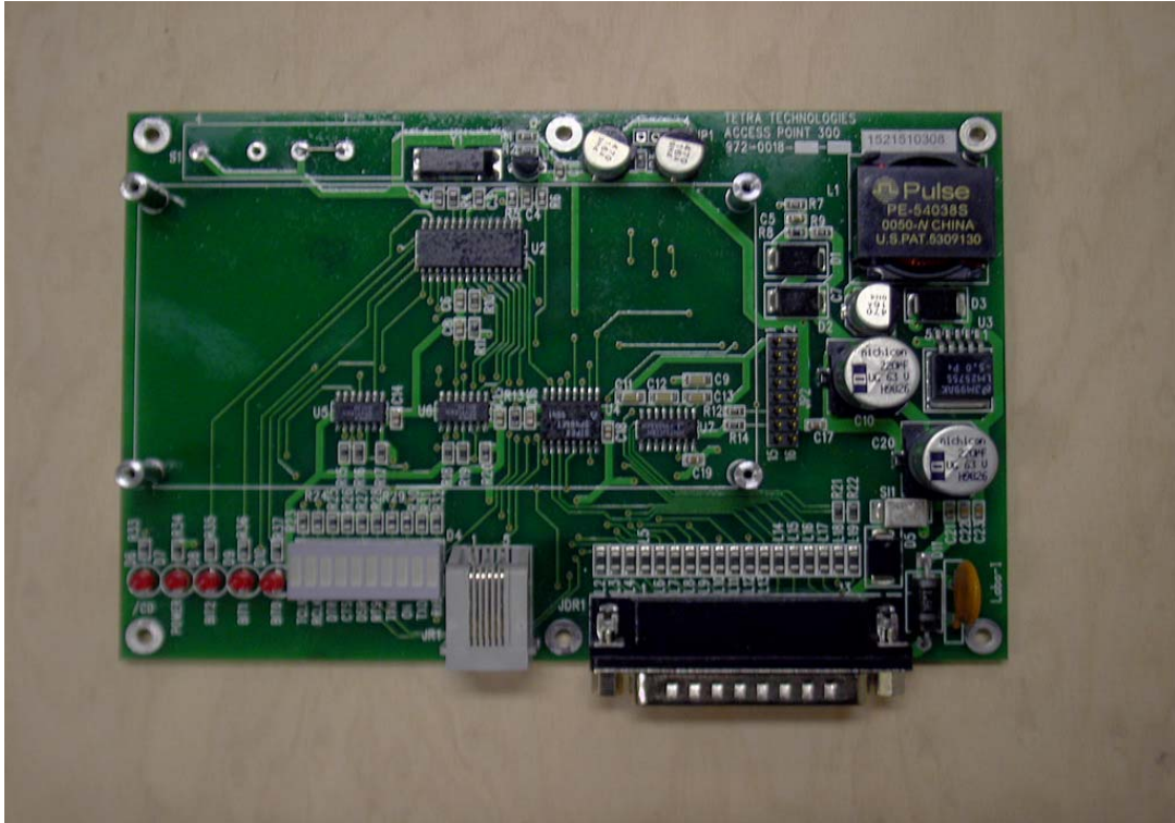
Photograph 5 - 2: Top Side of Main board.
