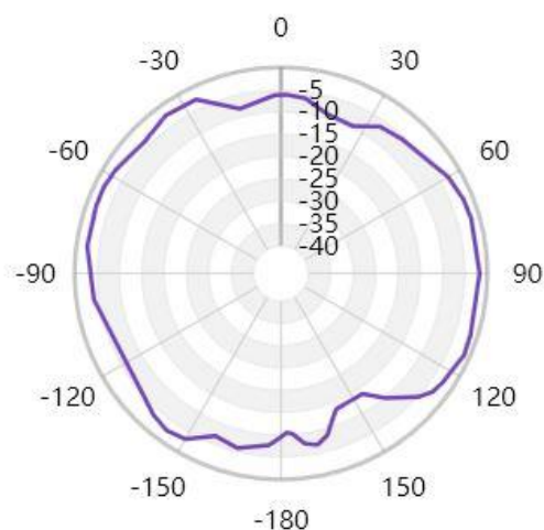
Free Space GAIN TOTAL (2480MHz) - XZ cut
