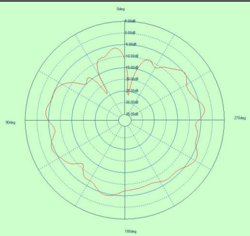
Free Space GAIN TOTAL (2480MHz) - XY cut
