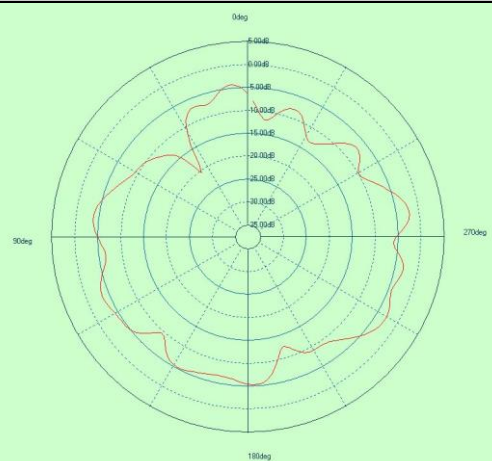
Free Space GAIN TOTAL (2440MHz) - XY cut
