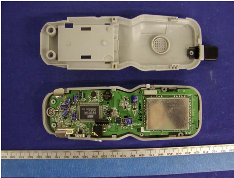
Base – Chassis Cover off View
