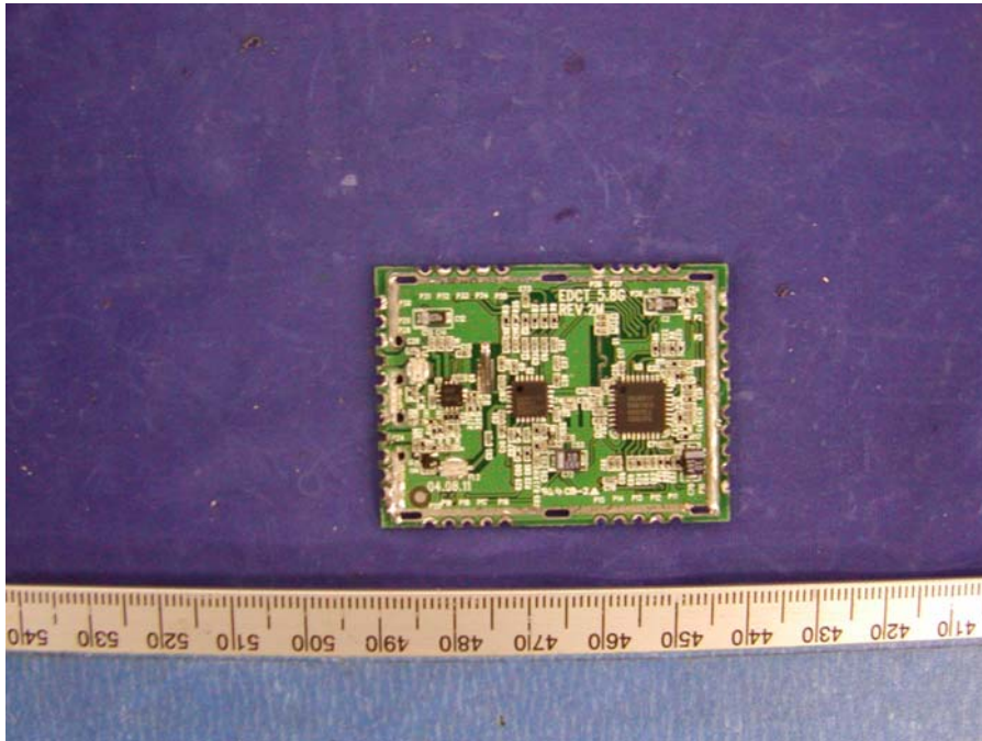
Base – Transceiver Bottom View
