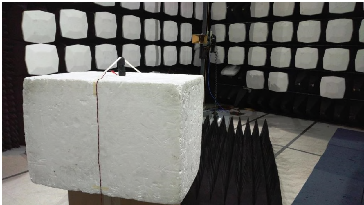
Figure 7: Equipment Under Test – Radiated Emissions >1GHz
