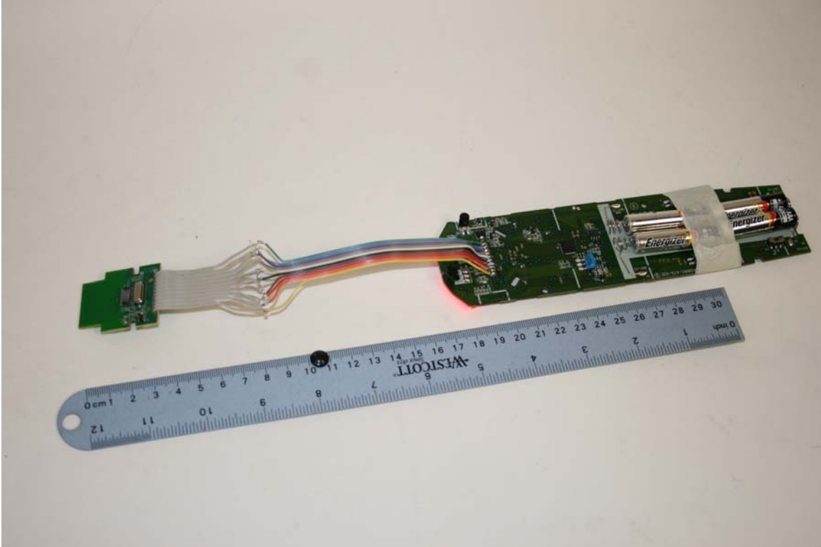
Ribbon cable extended for Modular Approval requirement of \geq 10\text{cm}
