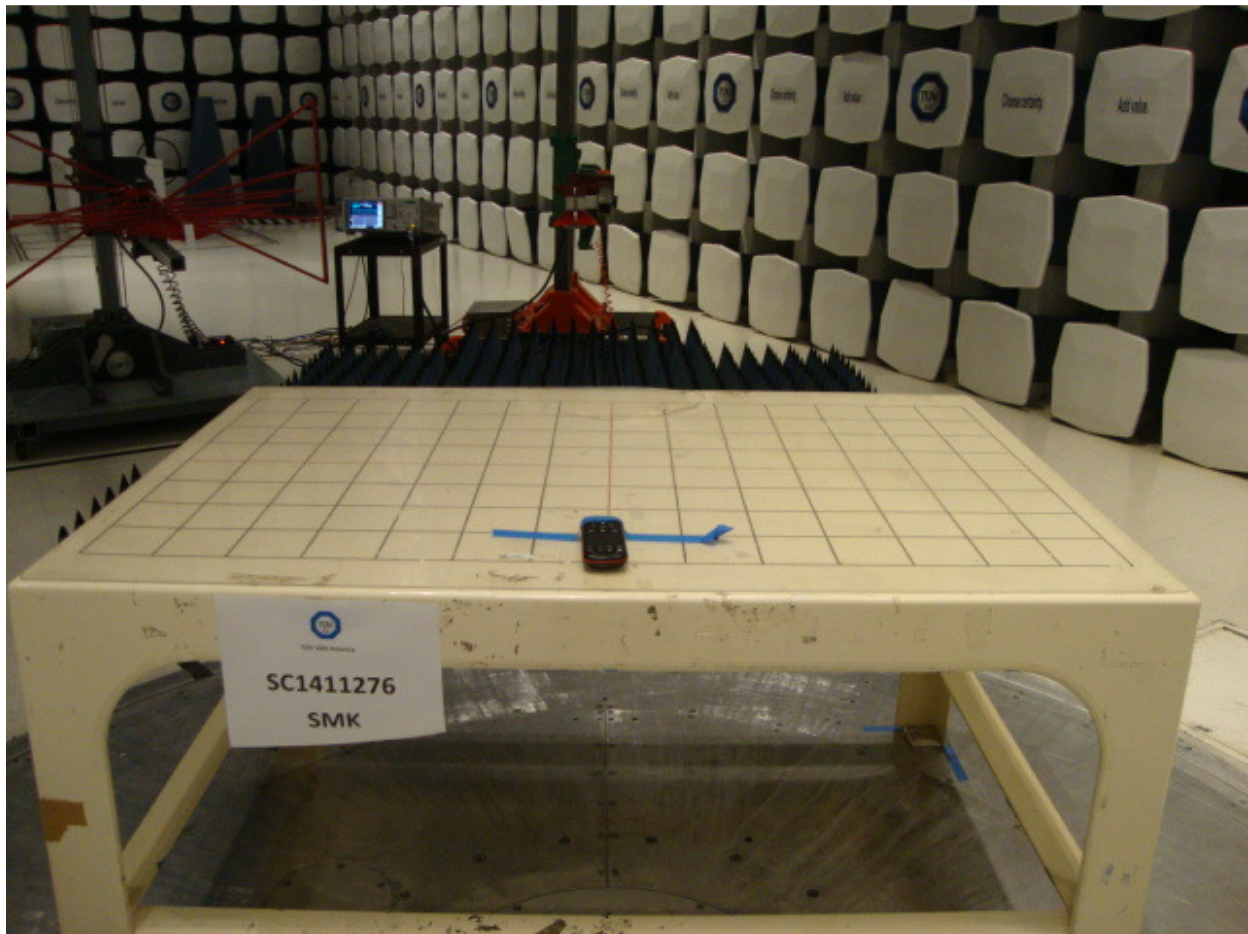
Figure 2 (1GHz-18GHz Rear Picture)
