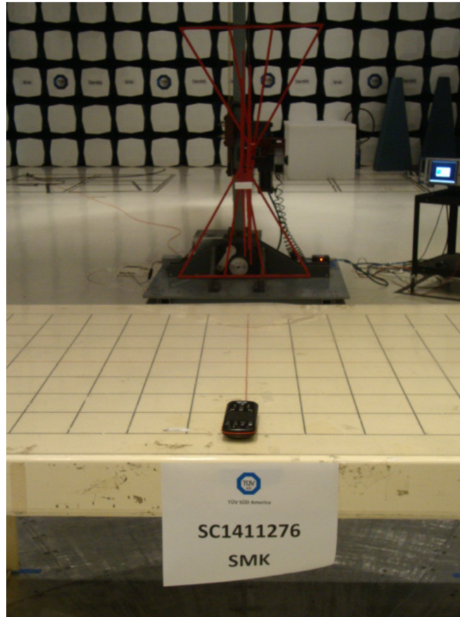
Figure 1(30MHz-1GHz Rear Picture)
