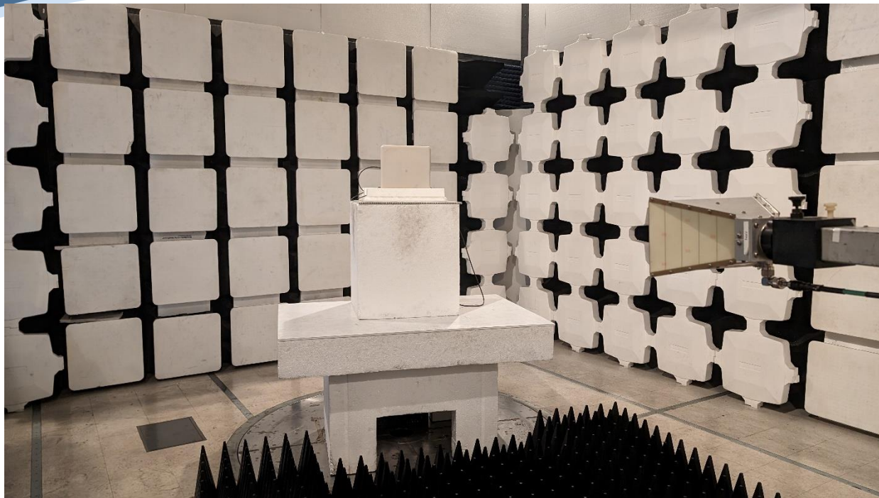
Spurious Emissions Panel 1-18GHz
