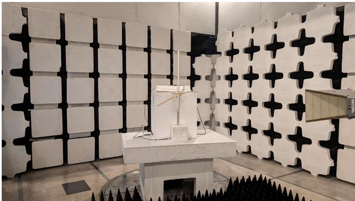
Spurious Emissions OMNI 1-18GHz
