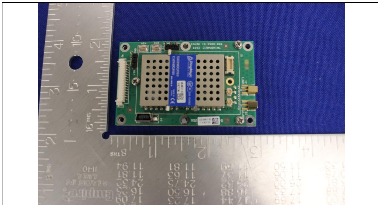
RF module soldered to Carrier board top with shielding view
