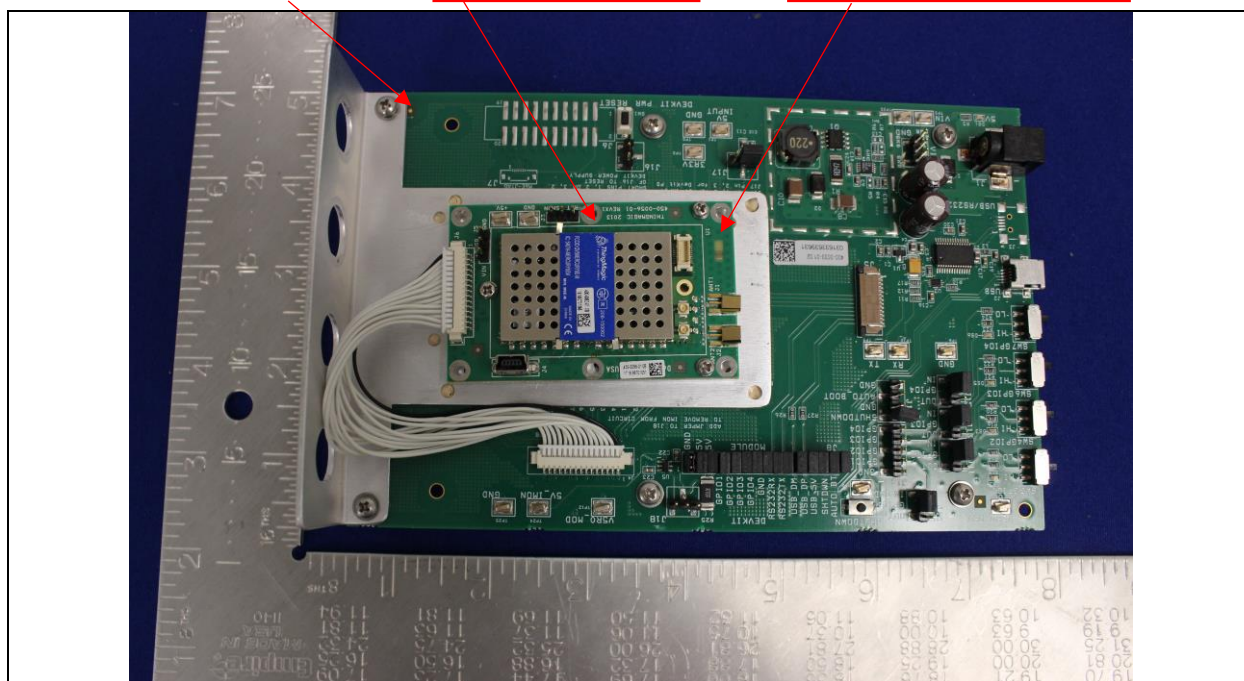
EUT soldered to carrier board with M6E-DEVKIT Top View
