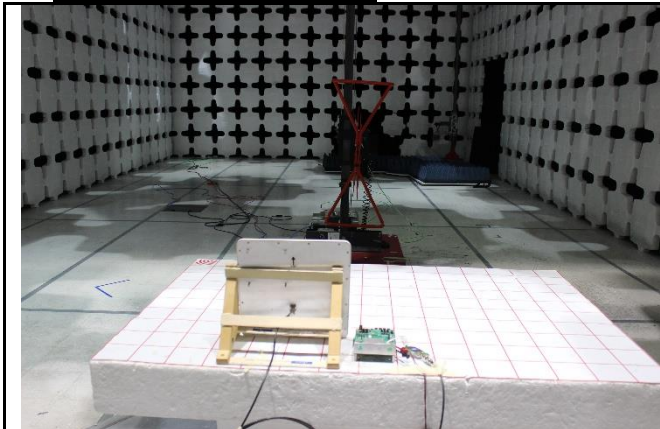
Radiated Emission Below 1G – Front View
