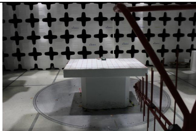
Radiated Emission Below 1G – Rear View
