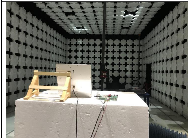
Radiated Emission Above 1G – Front View
