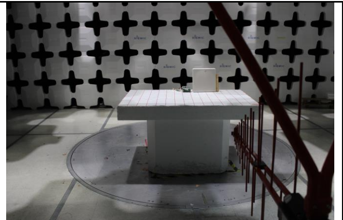
Radiated Emission Below 1G – Rear View
