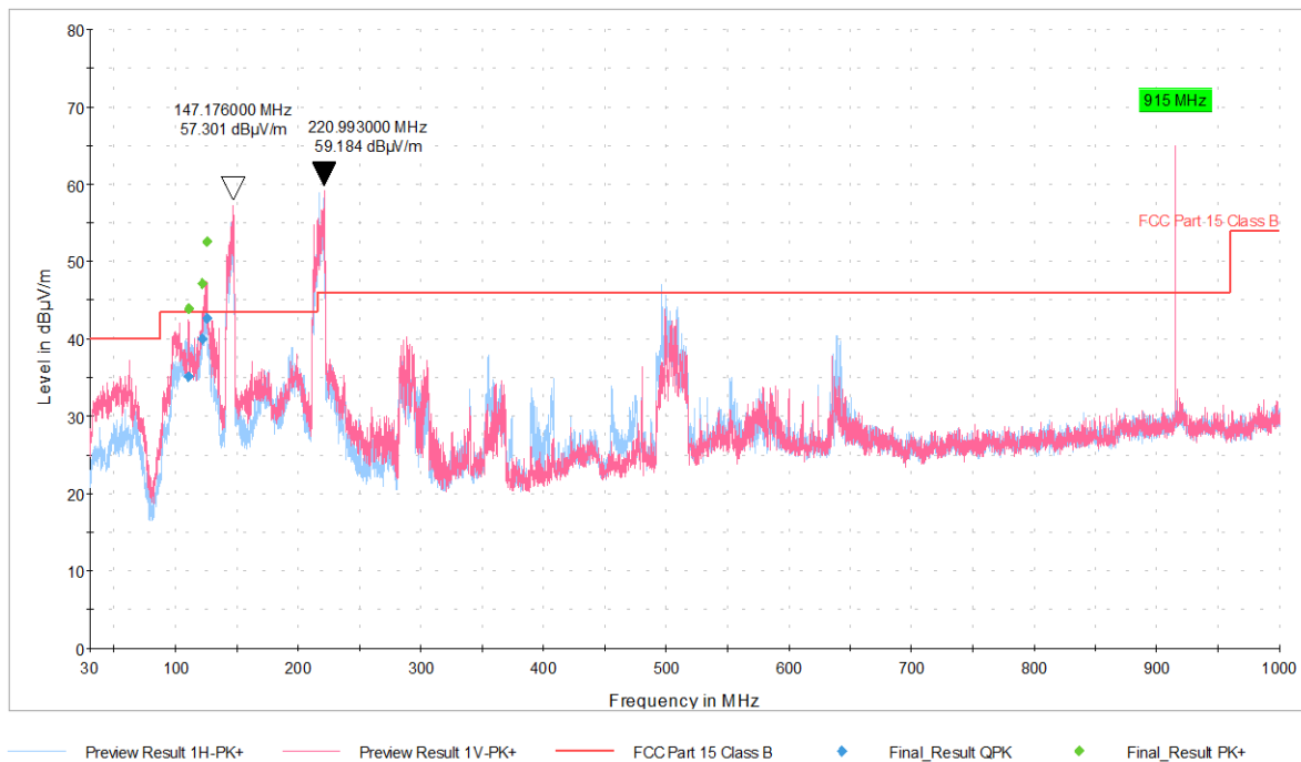
Figure 4. 30MHz-1GHz, 915 MHz
