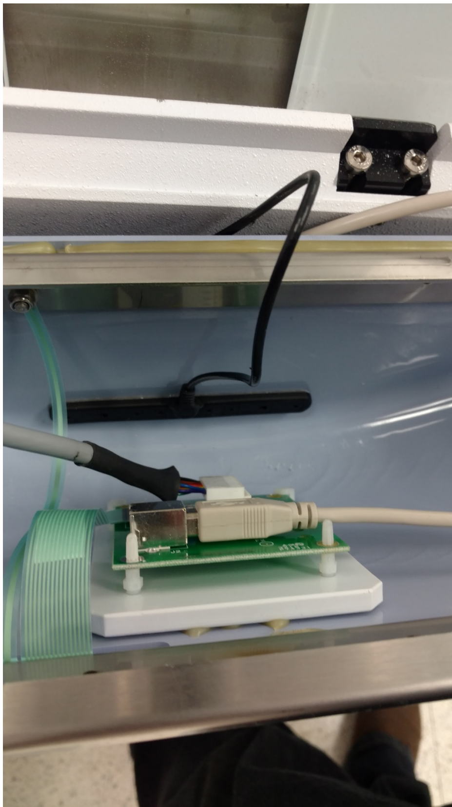
Figure 7 Dirty side RFID antenna
