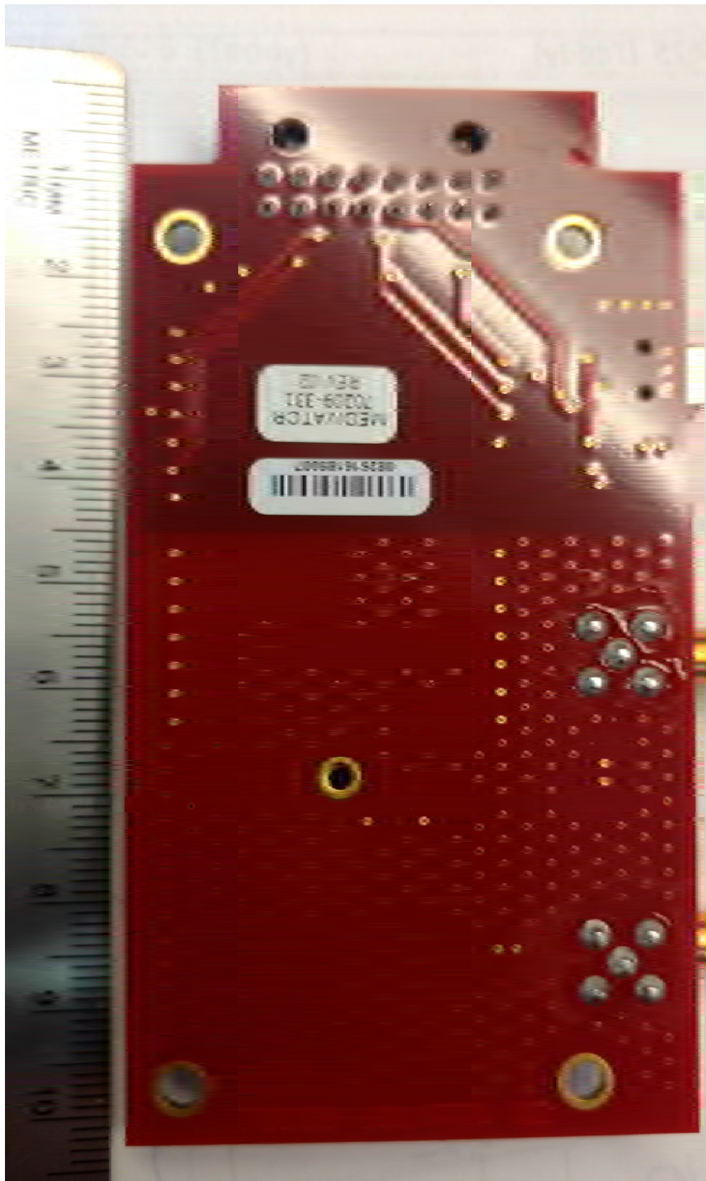
Figure 3 Bottom view of RFID carrier board
