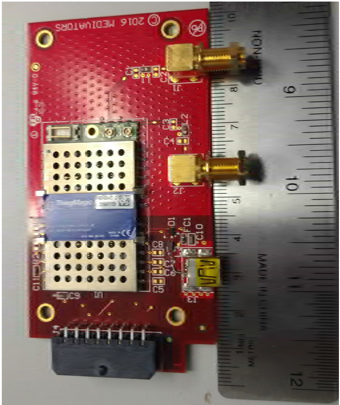
Figure 1 Top view of RFID carrier board with ruler
