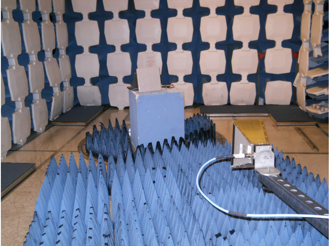
Spurious Emissions
