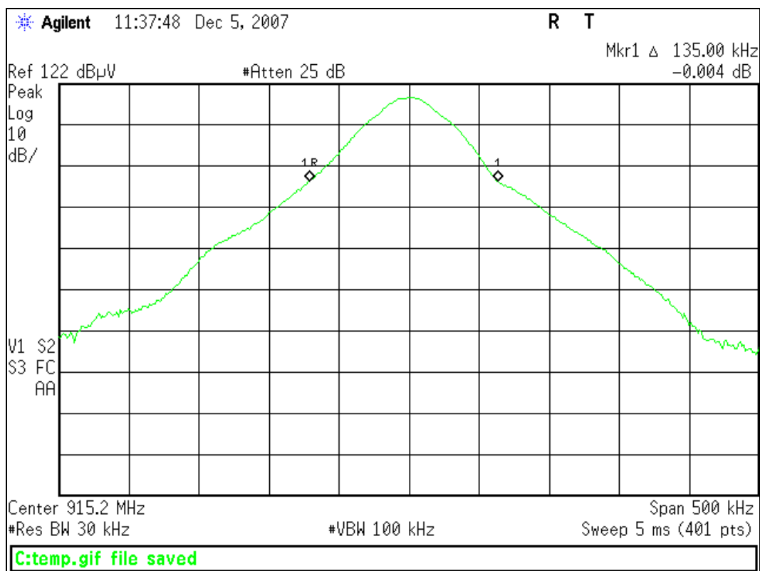
Channel 915.2MHz - 20dB Bandwidth
