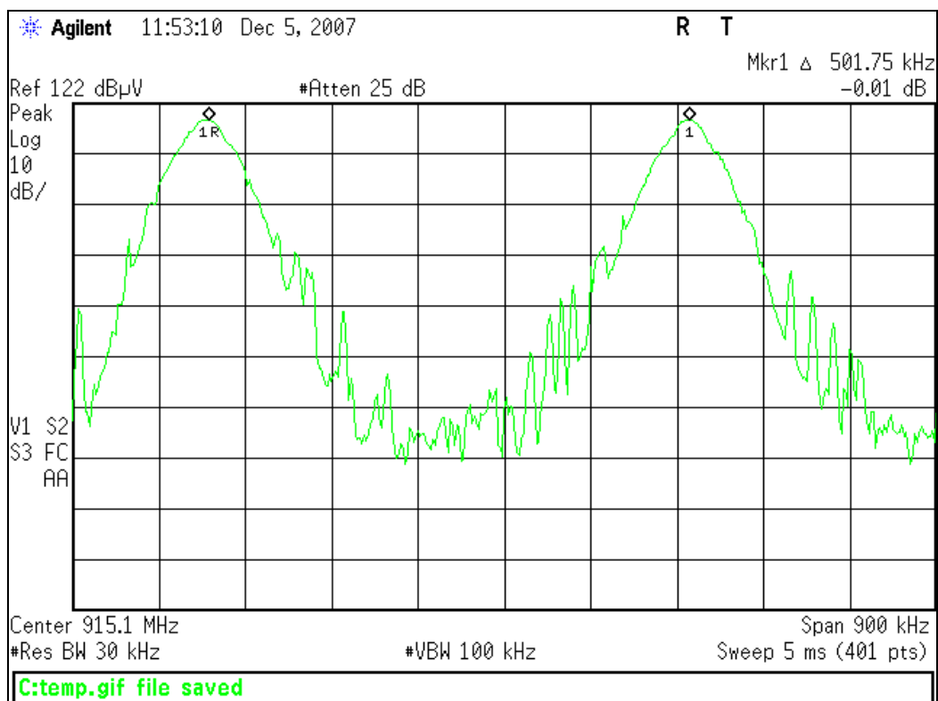
Channel 915.1MHz and Adjacent Channel - Channel Separation
