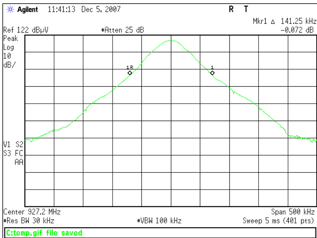
Channel 927.2MHz - 20dB Bandwidth
