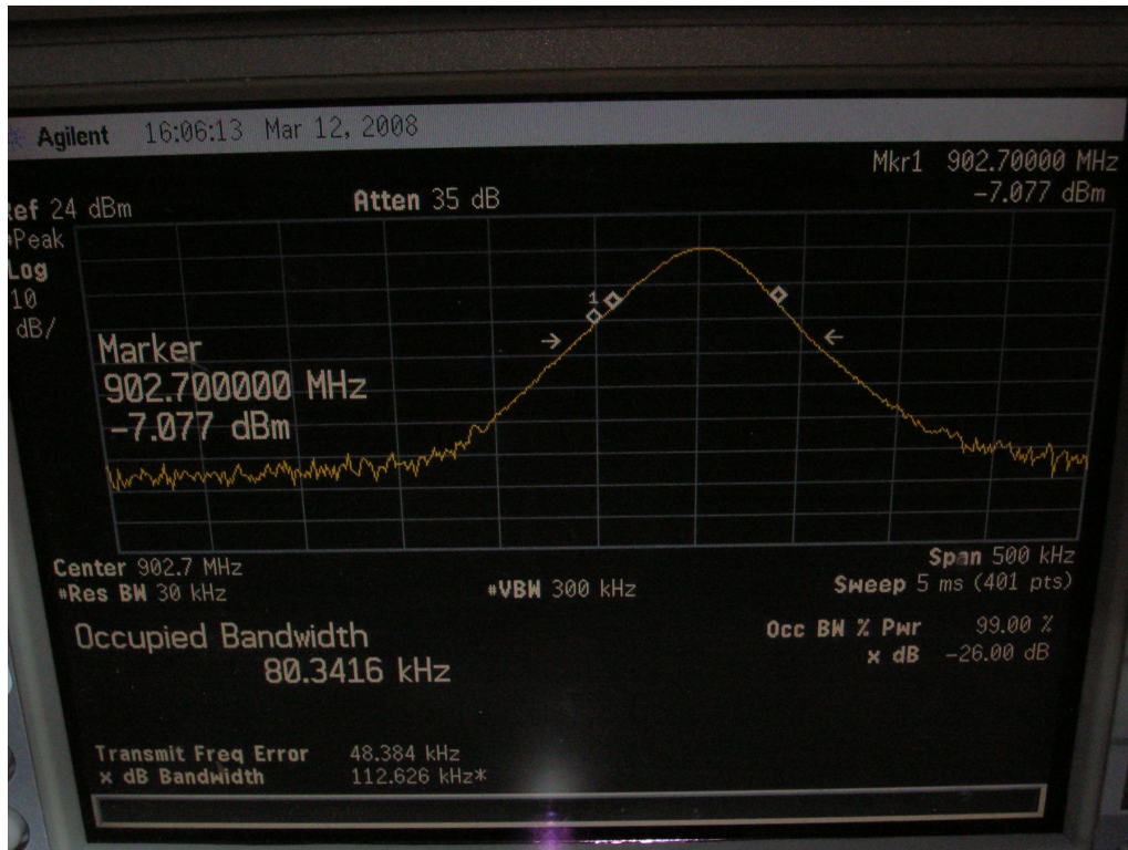
Channel 902.75MHz - 99% Occupied Bandwidth
