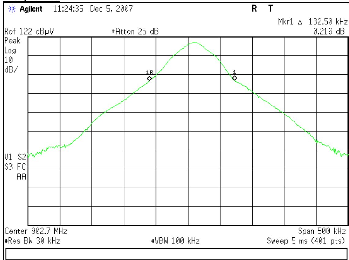
Channel 902.75MHz - 20dB Bandwidth
