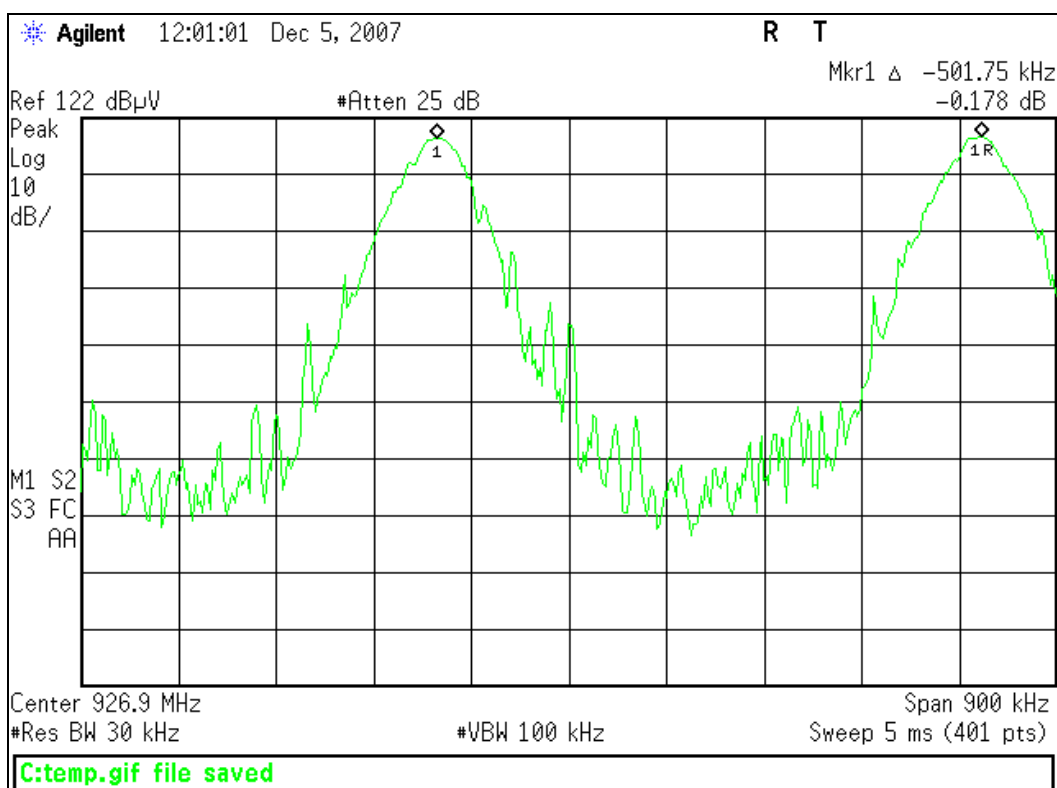
Channel 926.9MHz and Adjacent Channel - Channel Separation
